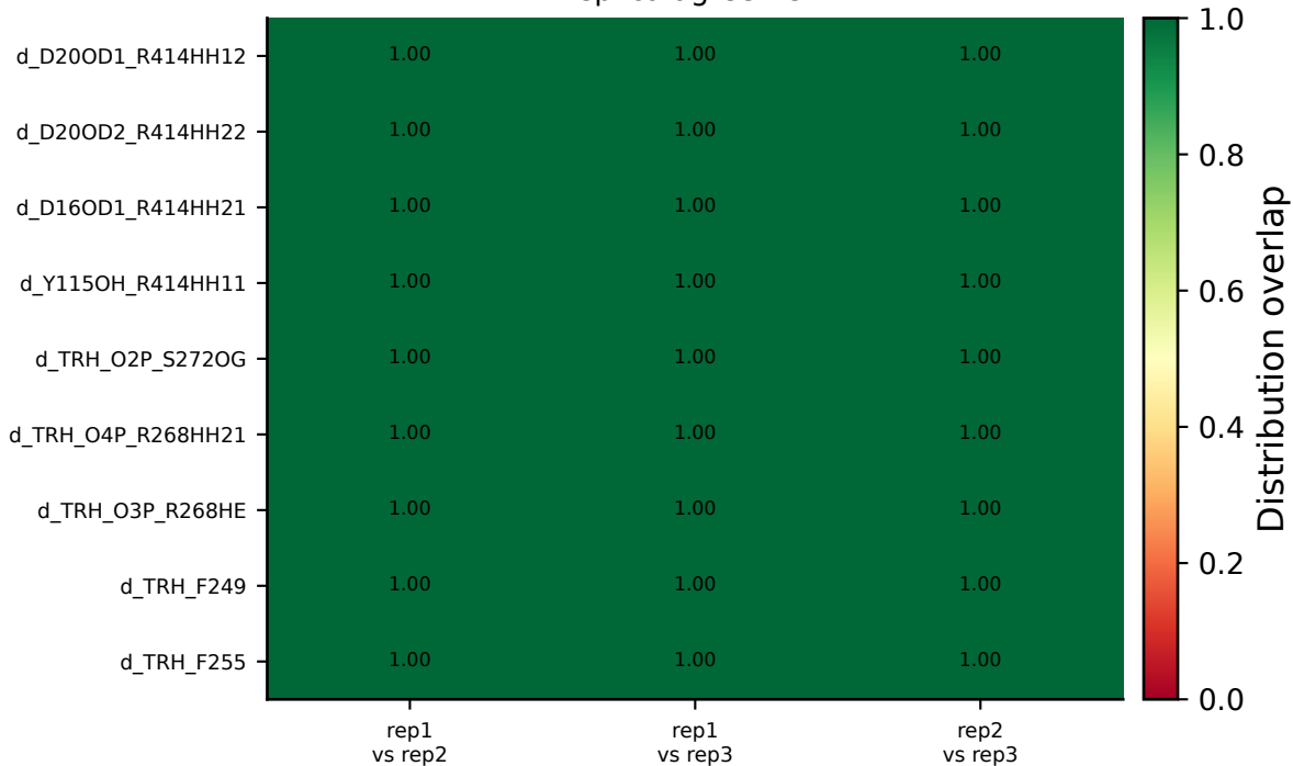
Replica agreement
