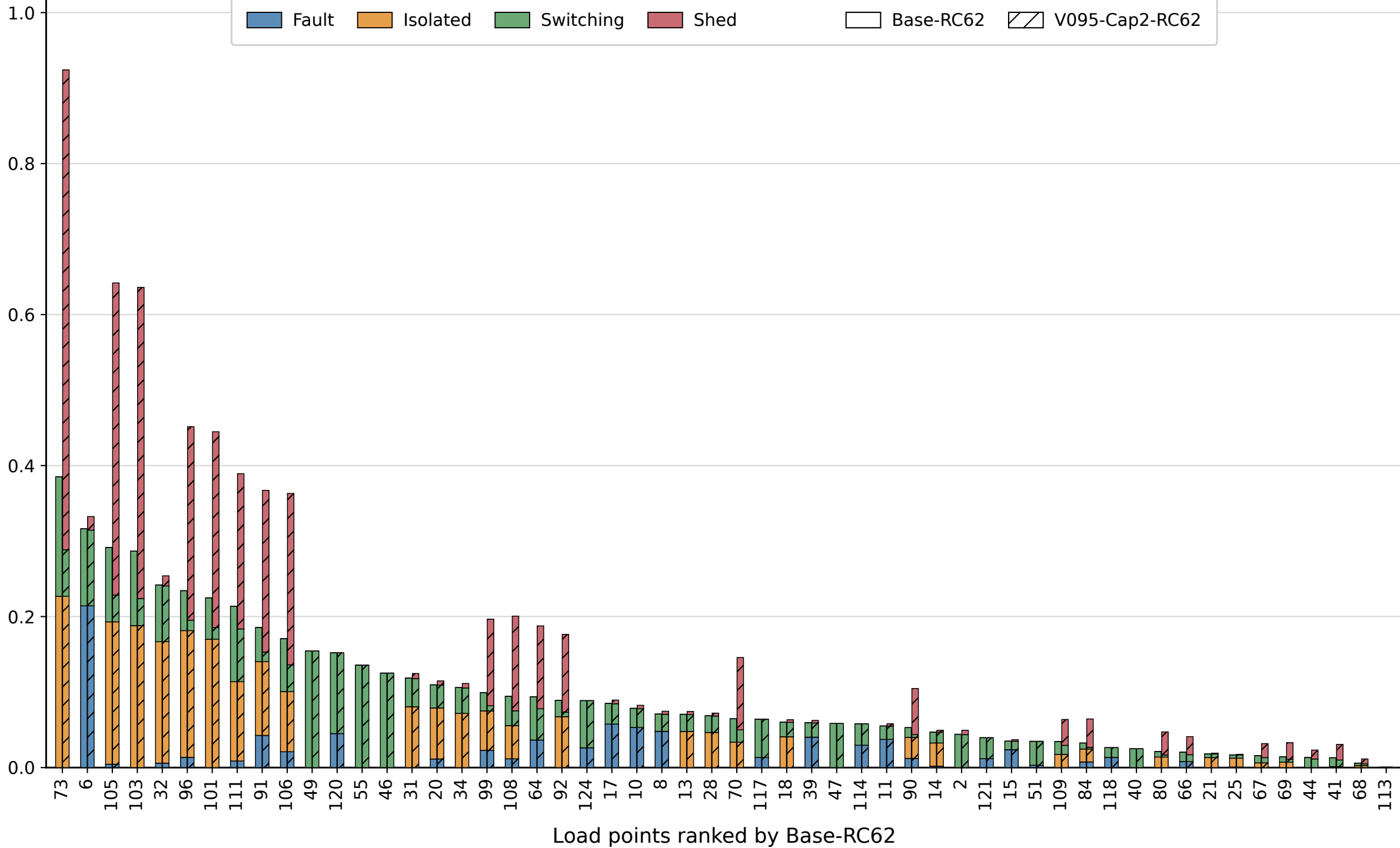
ENS breakdown [MWh/year]
