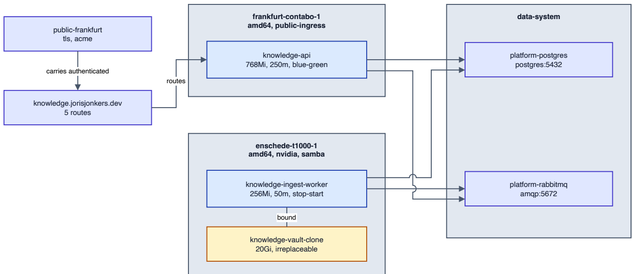
Figure 15: The knowledge Example's Resolved Model, as a Deployment View
