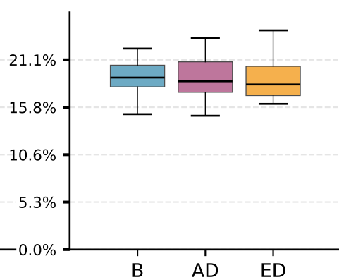
Space Invaders
