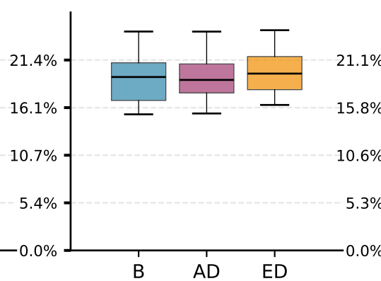
Seaquest
