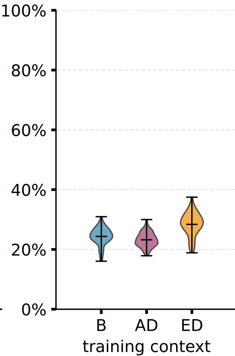
Breakout
