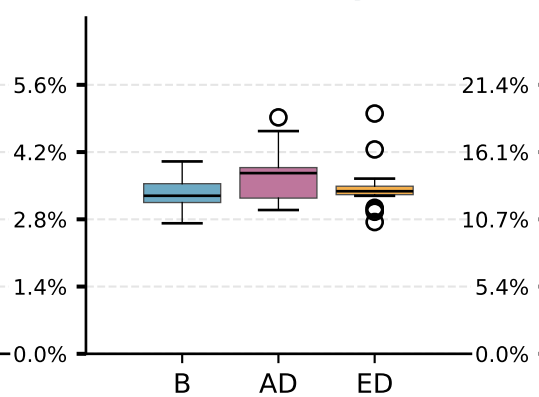
Freeway
