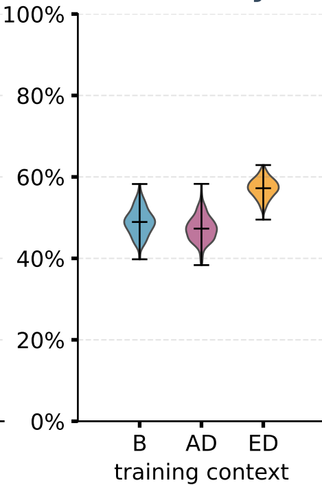
Freeway
