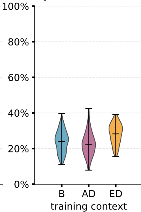
Space Invaders
