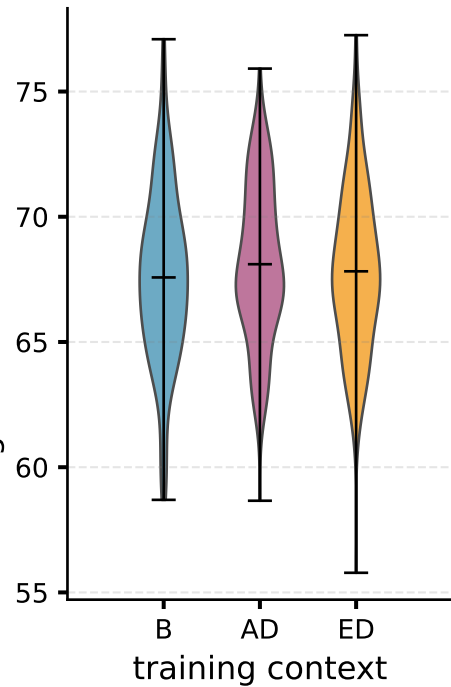
Asterix
