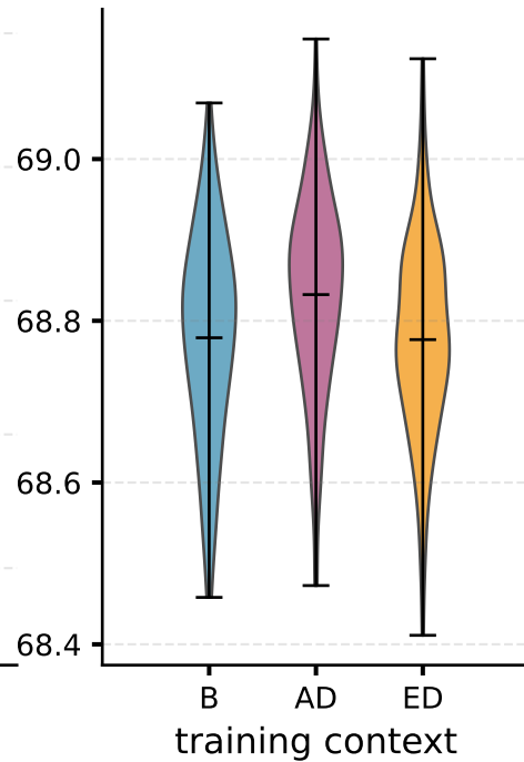
Freeway
