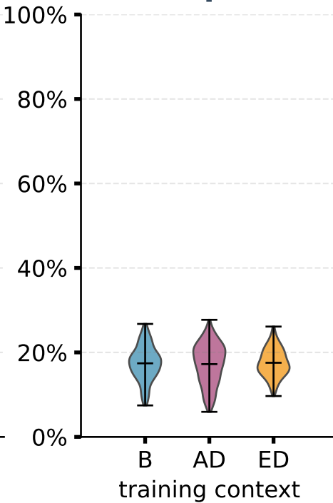
Seaquest
