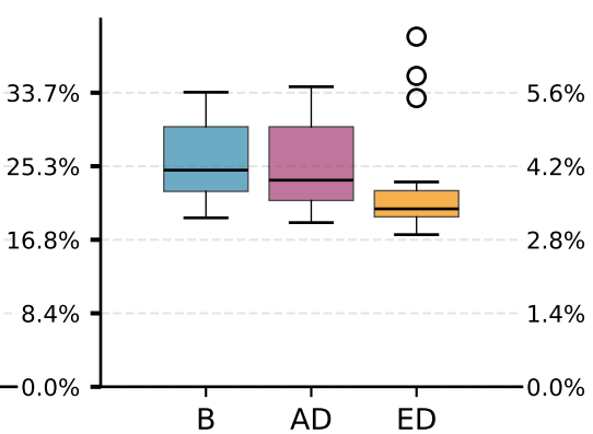
Breakout
