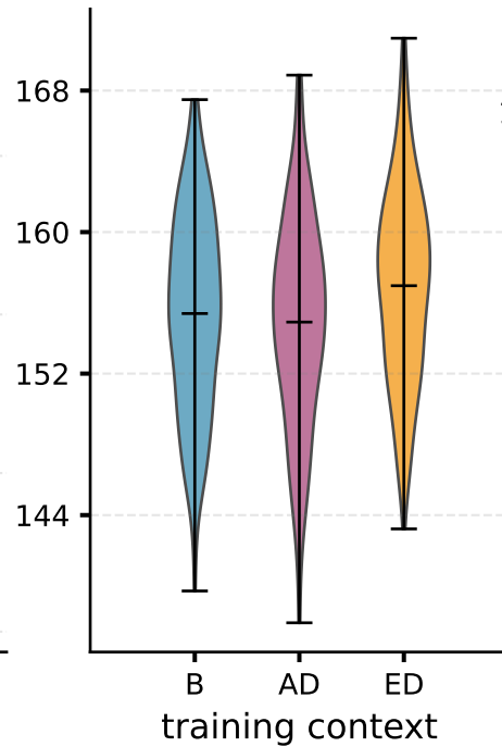
Seaquest
