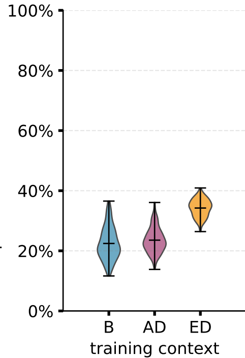
Asterix
