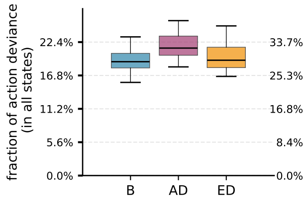
Asterix
