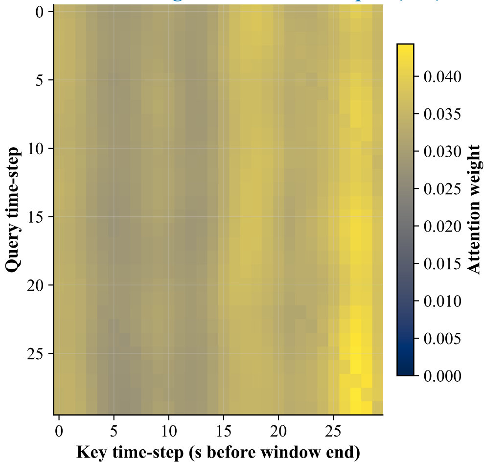
Mean Attention Weights — CLEAN samples (n=8)
