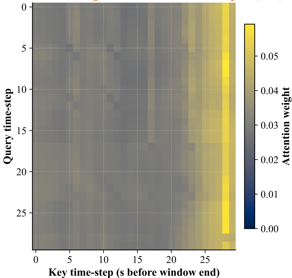
Mean Attention Weights — DEGRADED samples (n=8)
