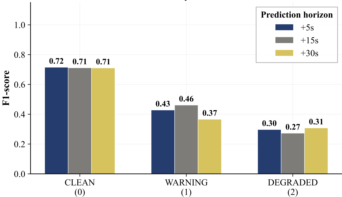
Per-class F1 Score by Prediction Horizon
