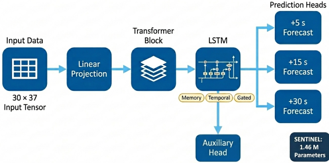
Figure 6: SENTINEL-GNSS architecture. A linear projection and positional encoding map the 30 by 37 input window to dimension 128. A two-layer Transformer encoder reads the window, a two-layer recurrent encoder with 256 hidden units summarises the sequence, and three heads output the class probabilities at the 5, 15, and 30 second horizons. The model has 1.46 million parameters.
