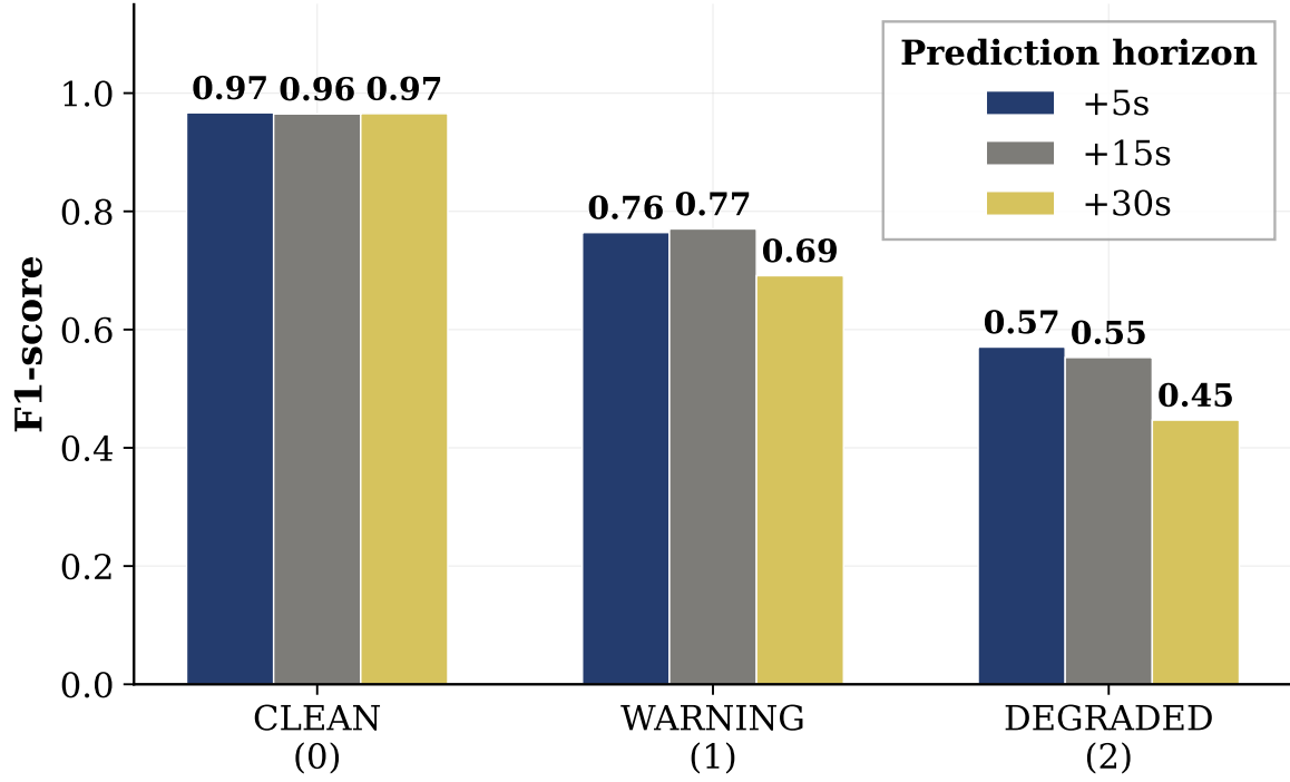
Figure 7: Multi-horizon Macro-F1 and per-class F1 comparison across all three prediction horizons. The +5s horizon achieves the strongest DEGRADED-class F1 and is used for real-time EKF integration.
