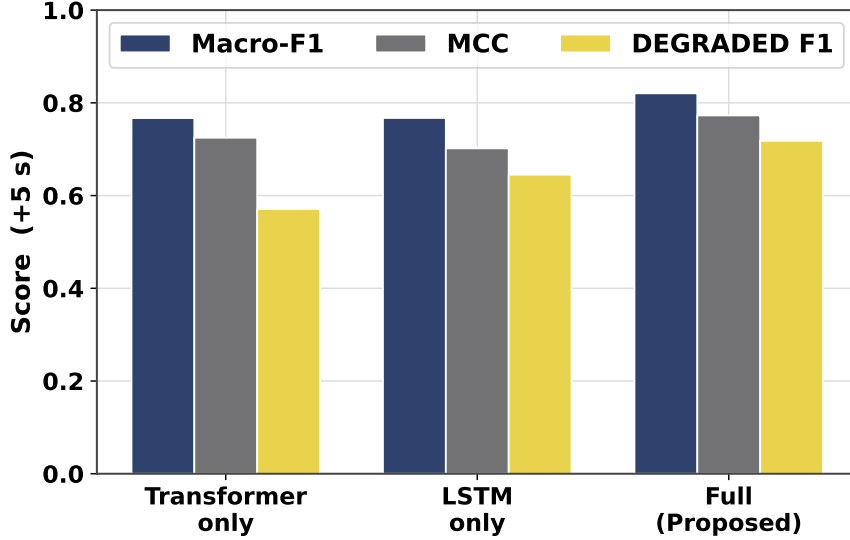
Figure 9: Ablation study: Macro-F1, MCC, and DEGRADED-class F1 for each architecture variant. Each component contributes independently.
