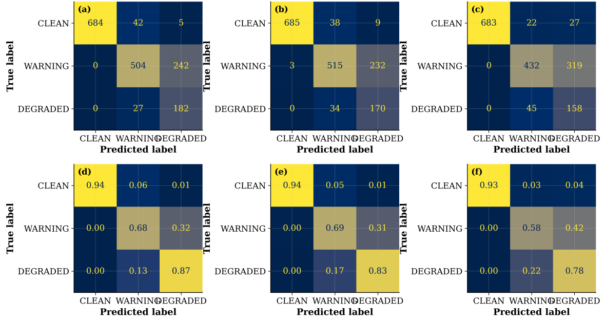
Figure 8: Confusion matrices for all three prediction horizons on the held-out test set. The +5s matrix shows strong DEGRADED recall with limited clean/warning confusion.
