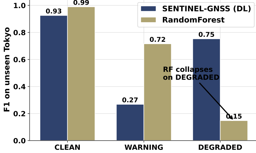
Figure 10: Cross-city DEGRADED-class F1 comparison. The DL model transfers to the unseen city; the RF baseline collapses, demonstrating the superiority of learned sequential representations for cross-environment generalisation.
