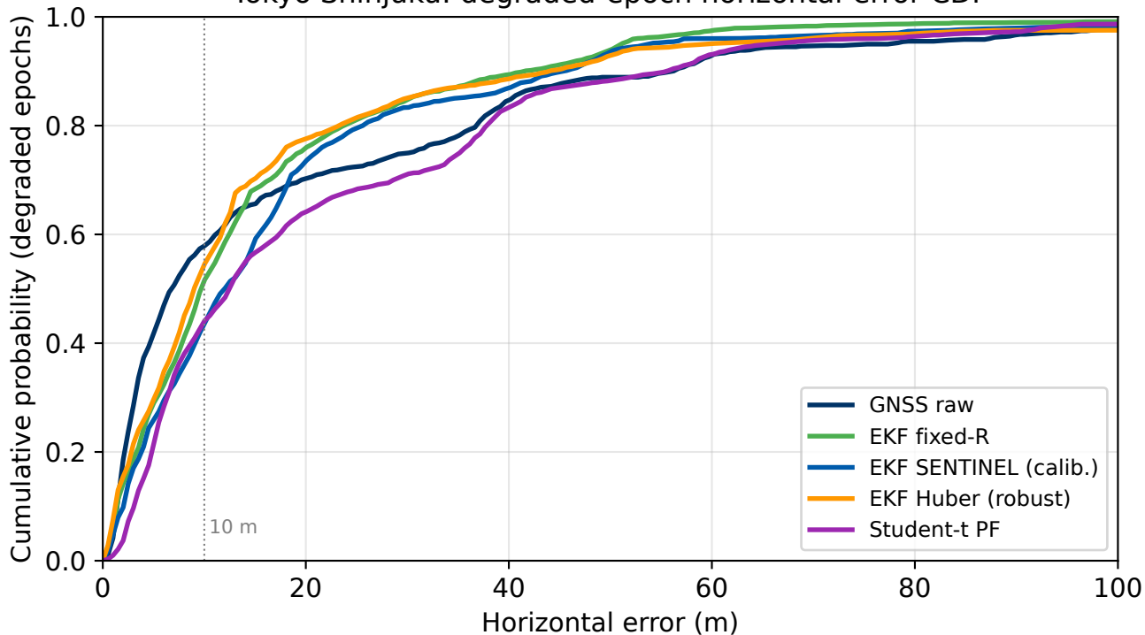
Tokyo Shinjuku: degraded-epoch horizontal-error CDF
