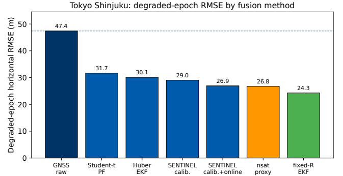
Fig. 5. Tokyo Shinjuku positioning RMSE comparison. The nine-state EKF provides consistently lower RMSE than the constant-velocity baseline. SENTINEL raw is hurt by receiver-domain shift; domain calibration restores it to 38.7% degraded-RMSE reduction, surpassing the robust-filter baselines and approaching the reactive proxy while providing proactive lead time.
