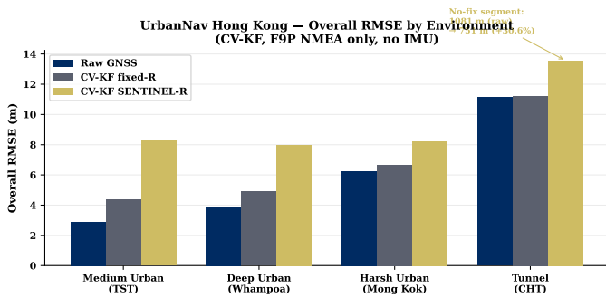
Fig. 7. UrbanNav Hong Kong results across four environments. SENTINEL improves over fixed- R dead reckoning only in the tunnel (30.6% no-fix RMSE reduction); in non-outage environments the high-quality F9P GNSS dominates and the constant-velocity EKF without IMU cannot help.
