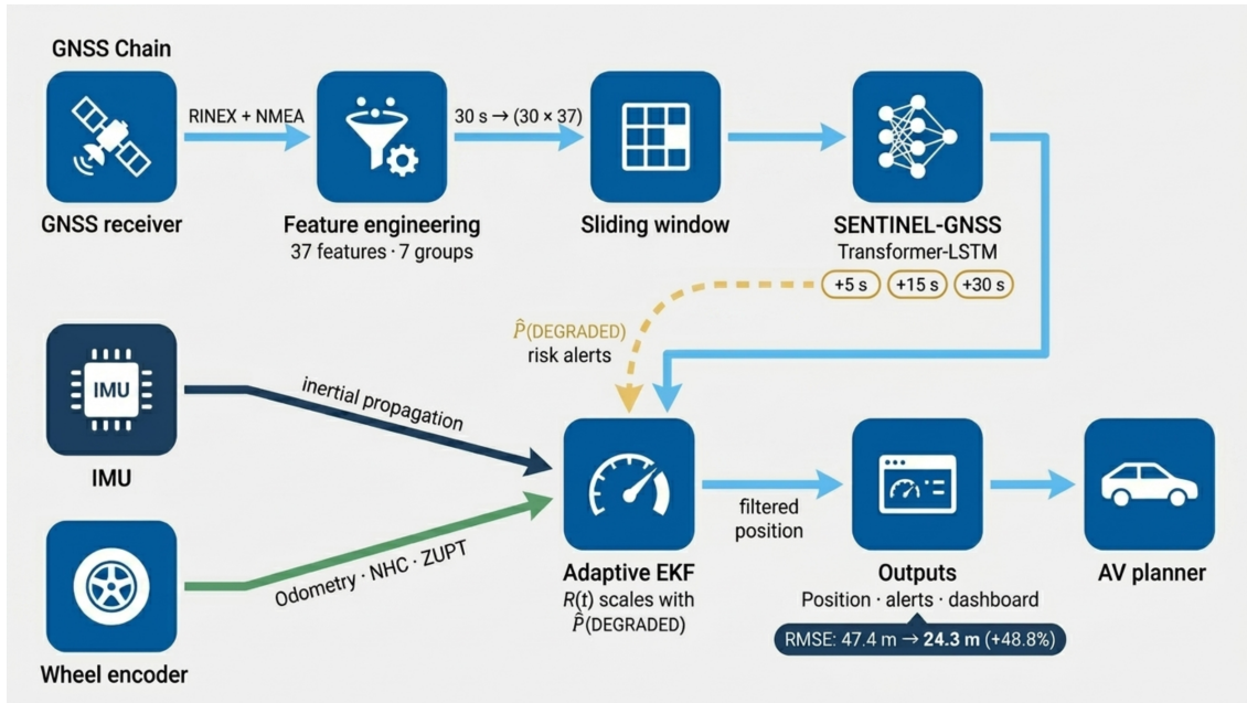
Figure 2: End to end SENTINEL-GNSS system. Sensors feed feature engineering, the model forecasts the degradation probability at three horizons, the Extended Kalman Filter scales its measurement noise with that probability, and the output layer produces position, alerts, and the dashboard view.
