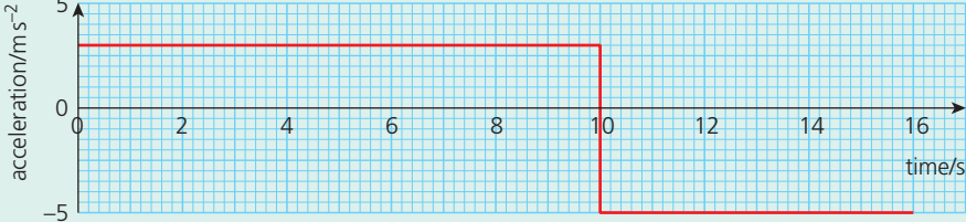
▲ Figure 2.20 Acceleration–time graph
