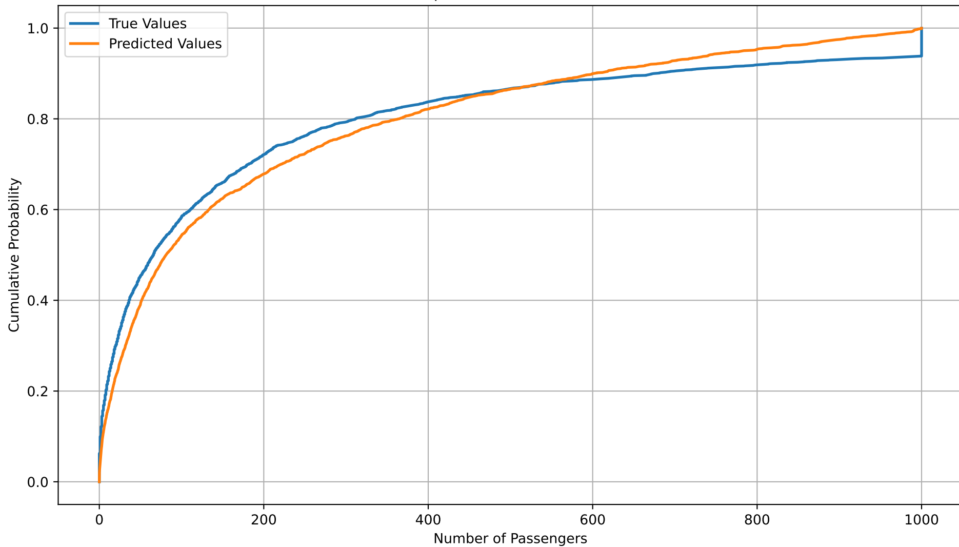
Random Forest: Empirical CDF of True vs Predicted Values
