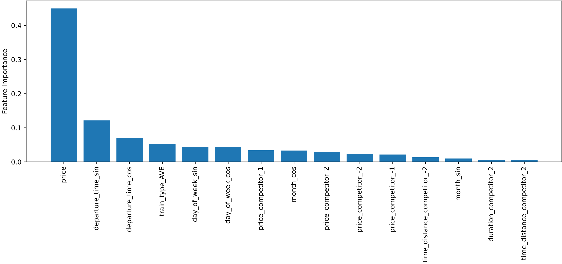
GBM: Top 15 Feature Importances
