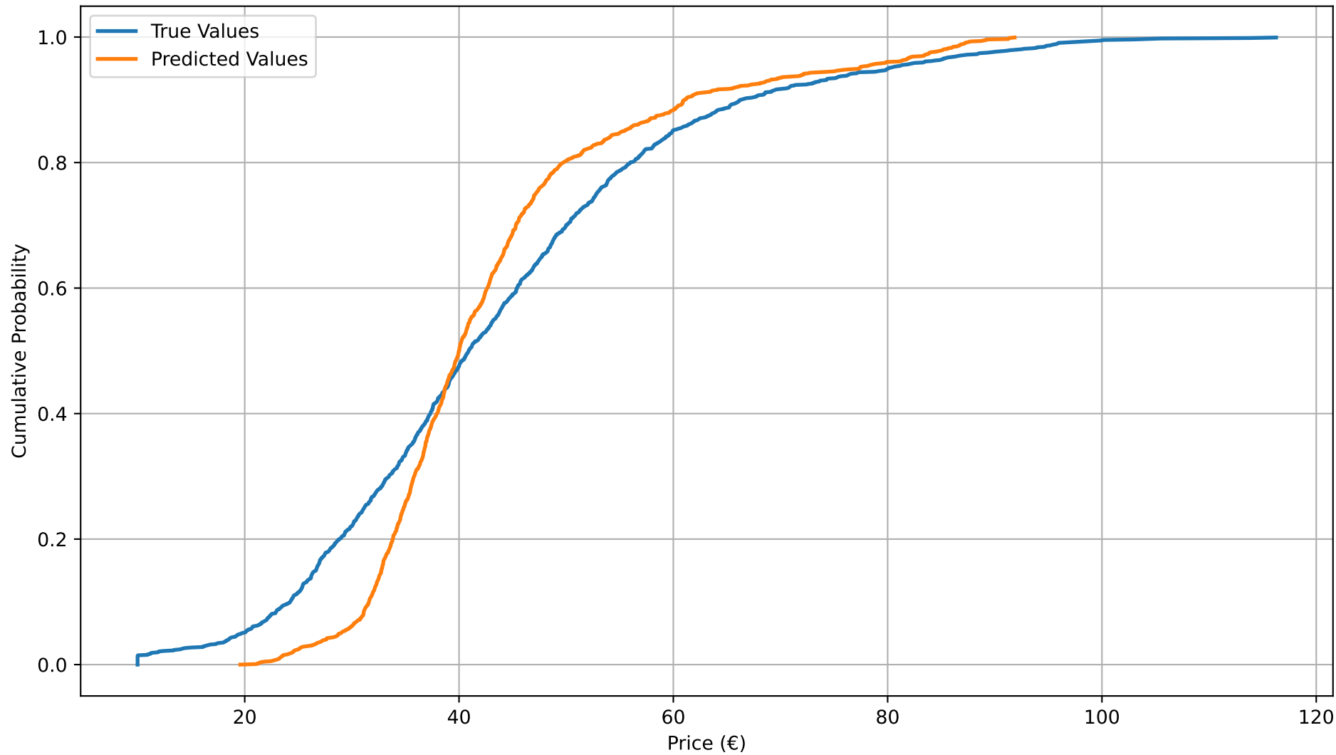
Price GBM: Empirical CDF of True vs Predicted Values
