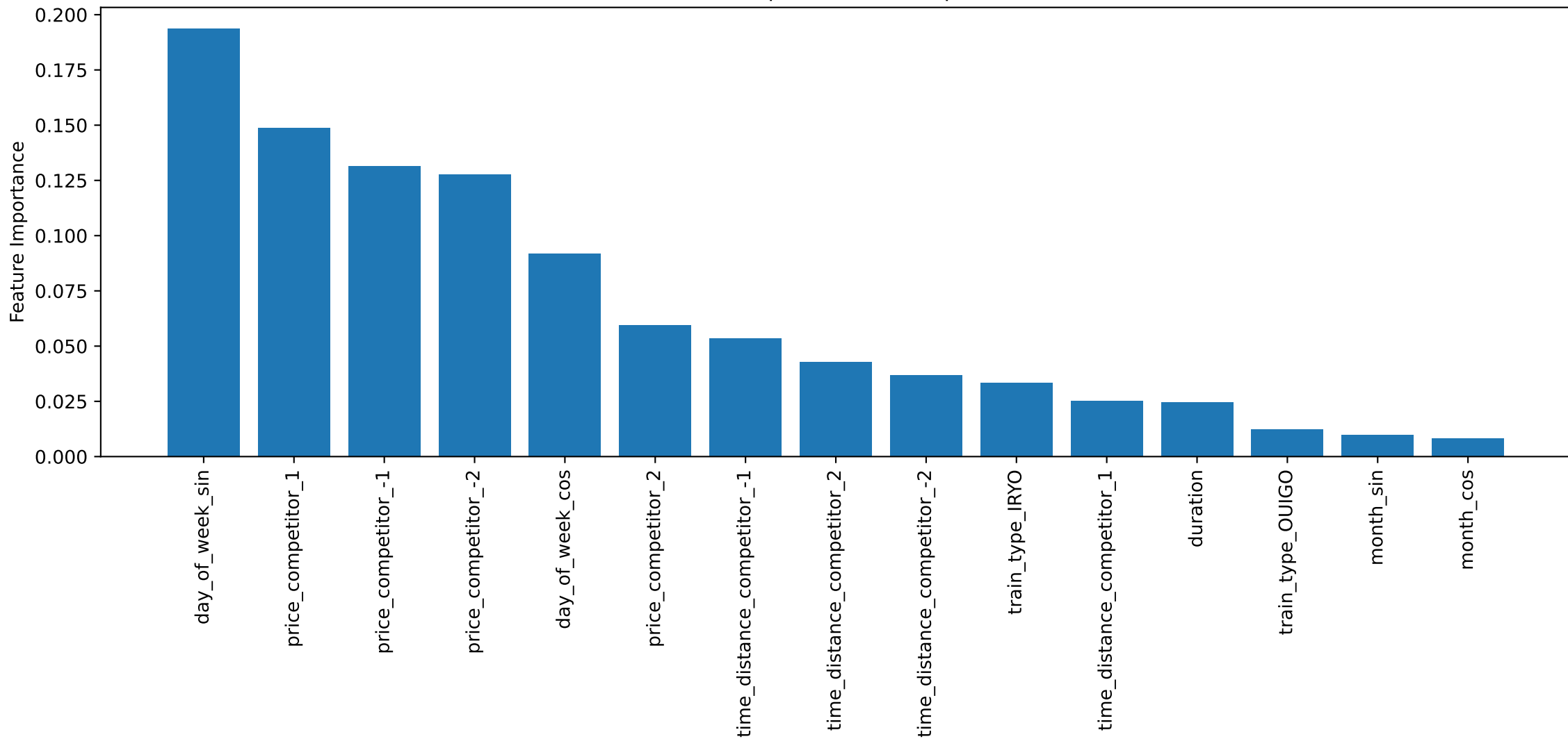
Price GBM: Top 15 Feature Importances
