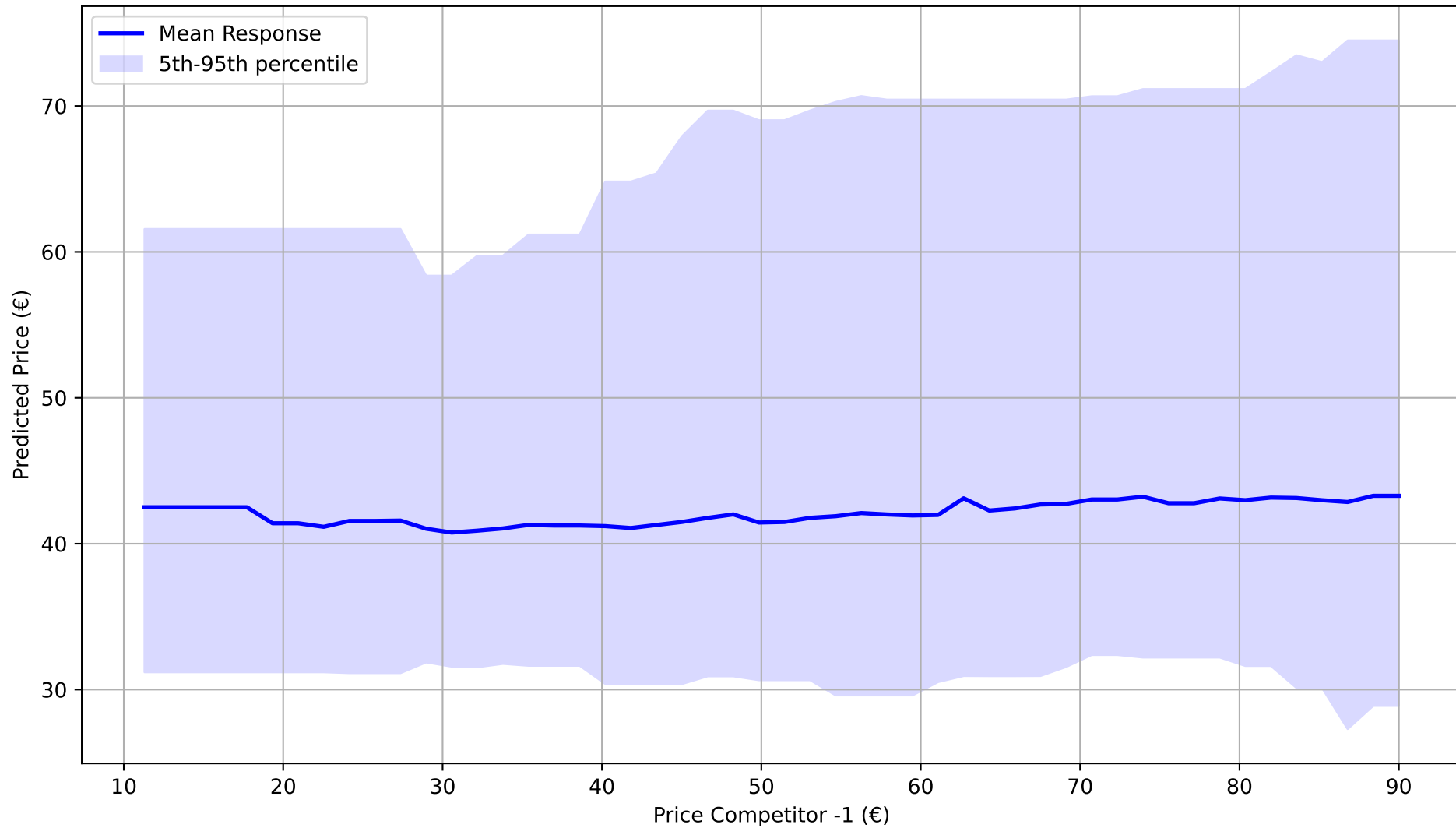
Price GBM: Partial Dependence on Price Competitor -1
