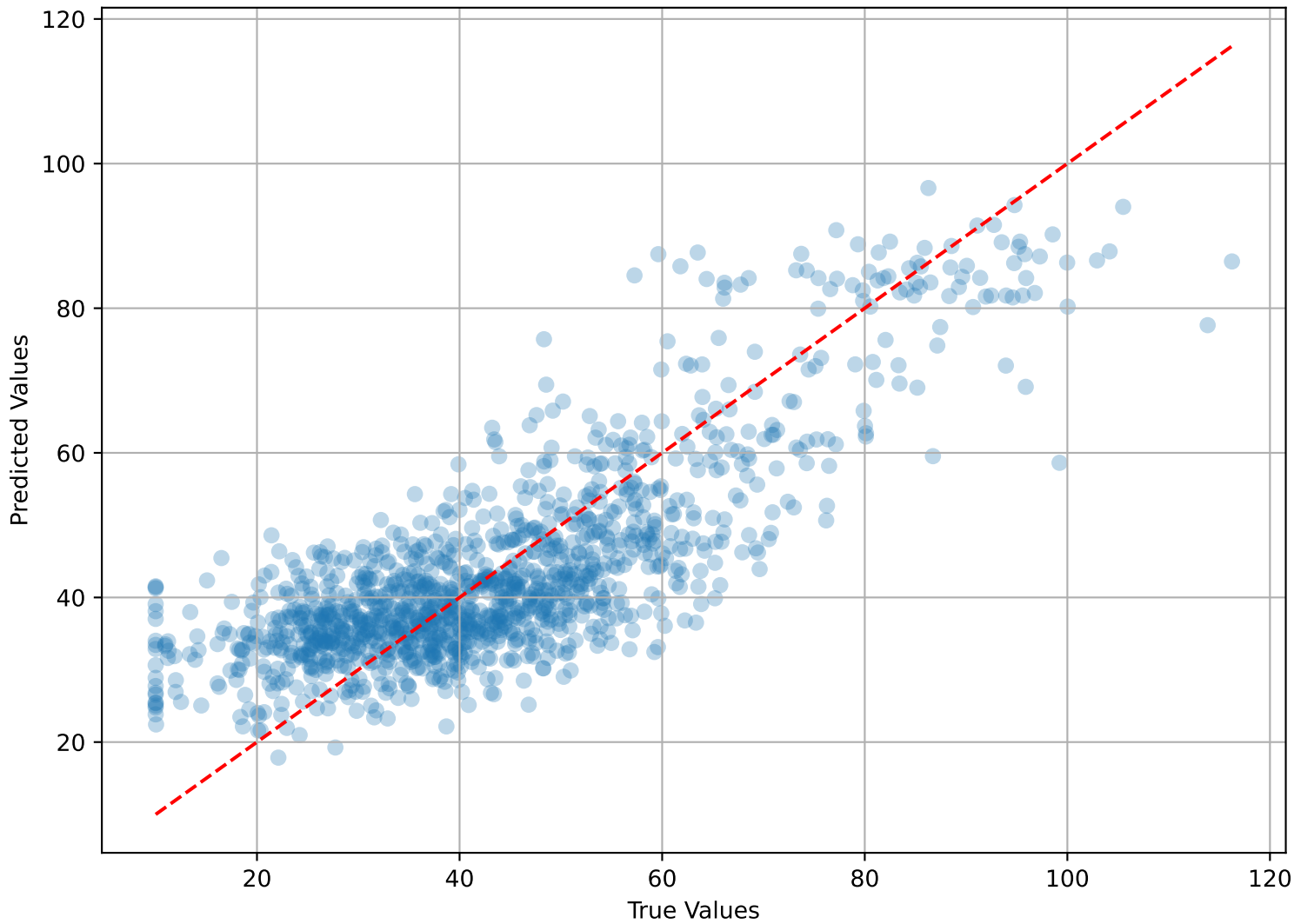
Price GBM: Predicted vs True Values
