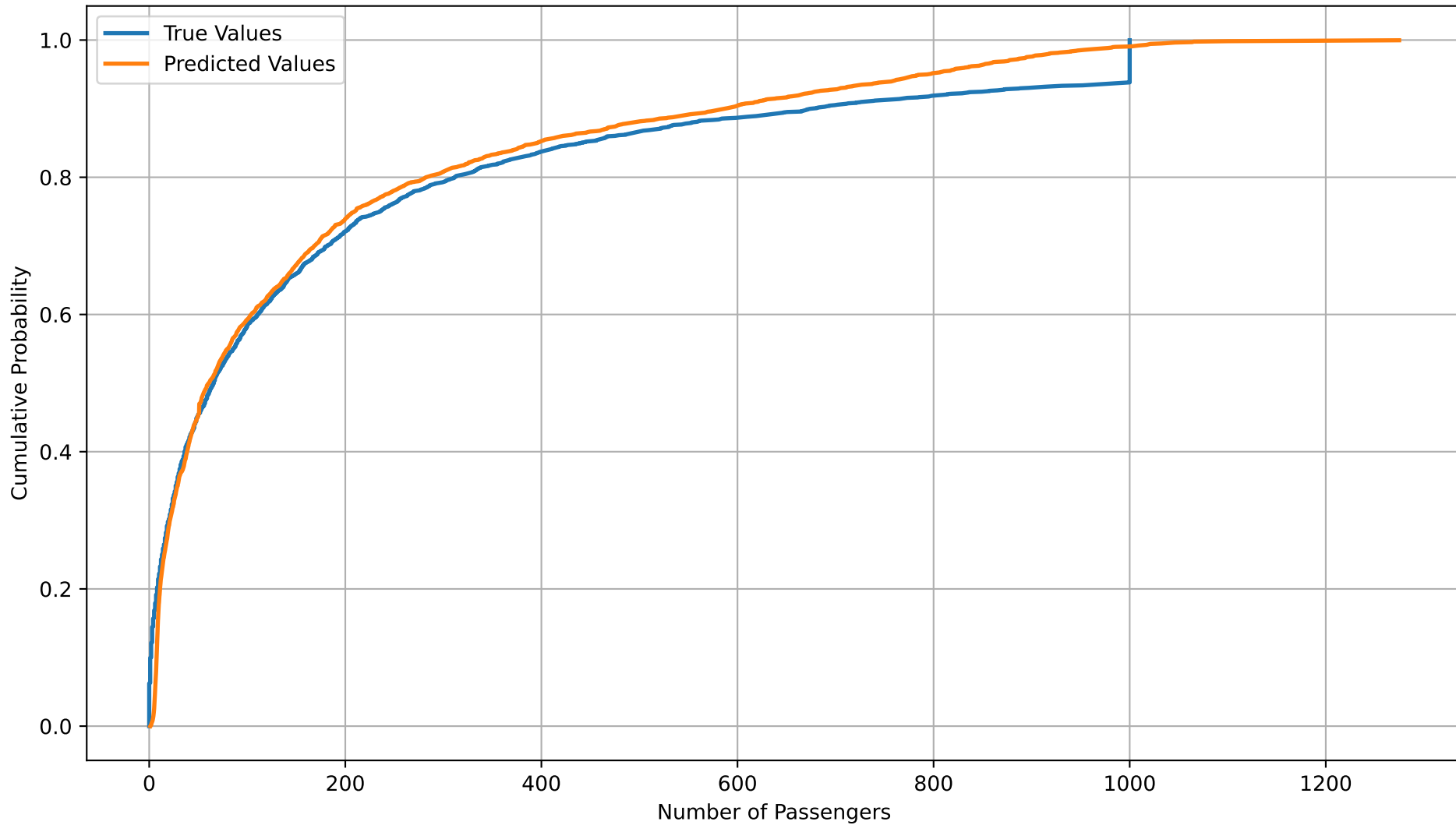
Empirical Cumulative Distribution Function (CDF) of True vs Predicted Values
