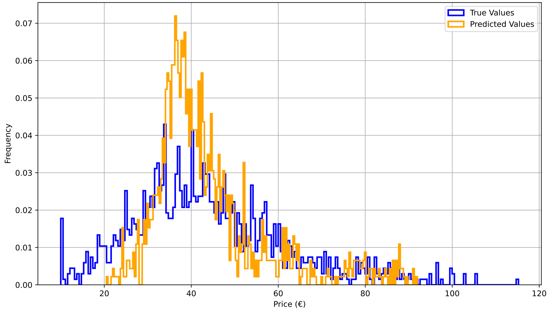
Price GBM: Histogram of True vs Predicted Values
