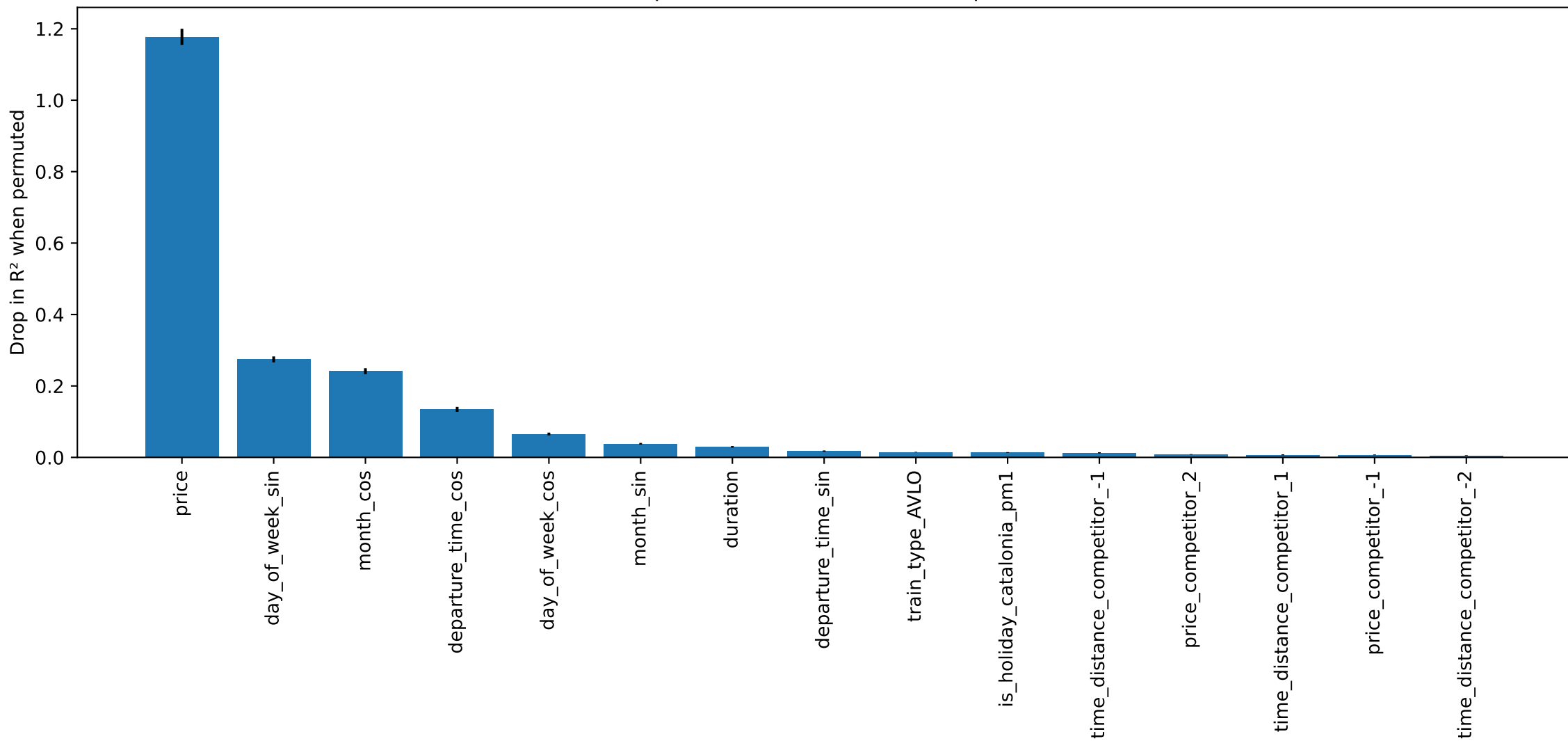
GBM: Top 15 Permutation Feature Importances
