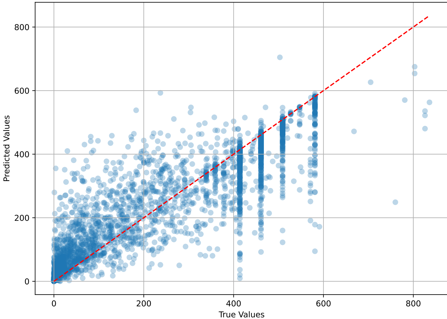
Random Forest: Predicted vs True Values
