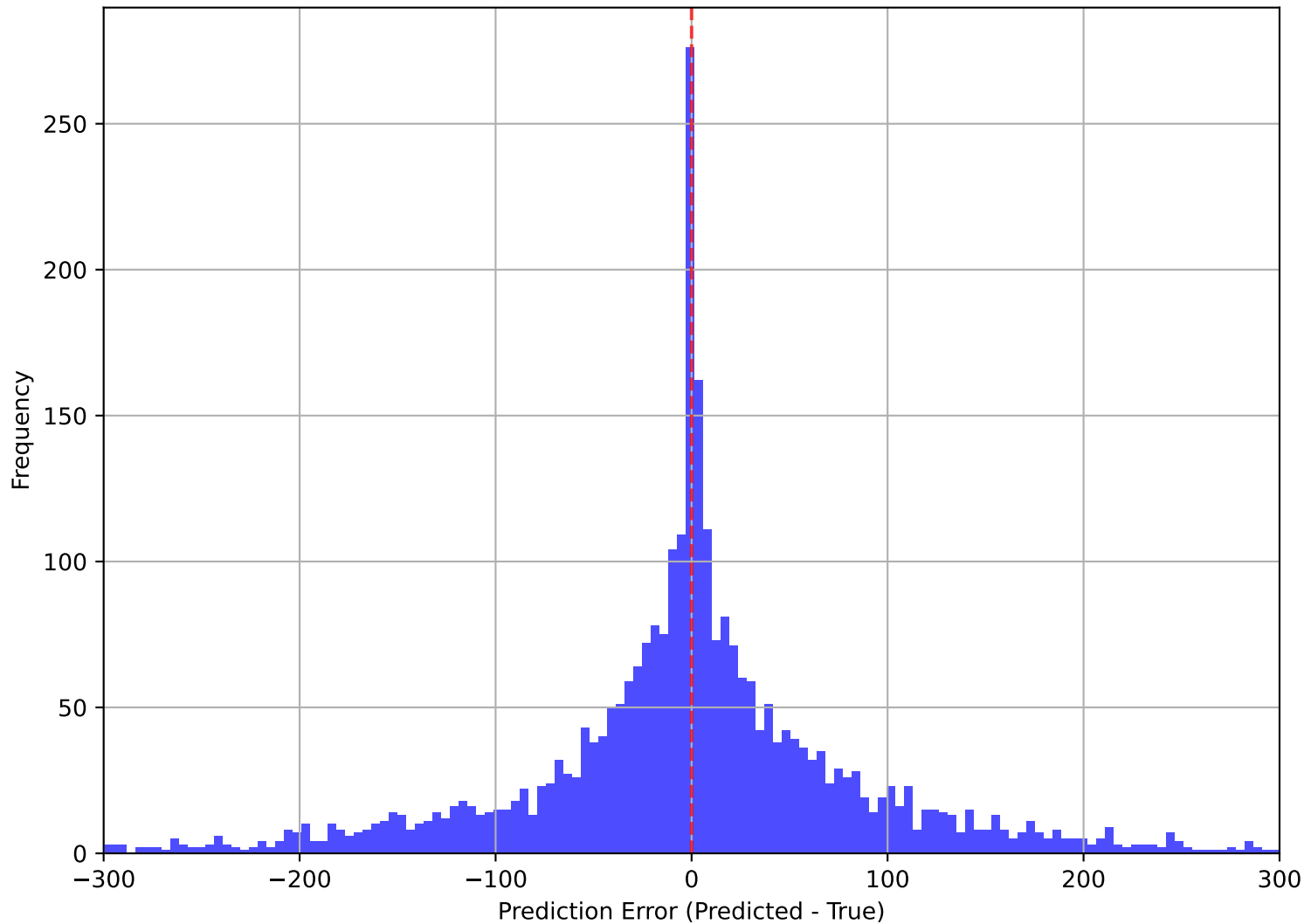
Random Forest: Histogram of Prediction Errors
