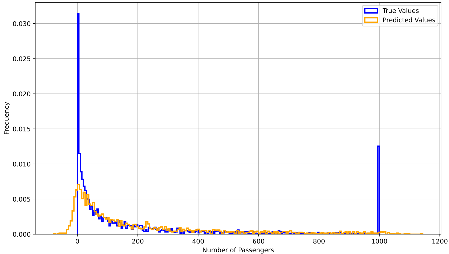
GBM: Histogram of True vs Predicted Values
