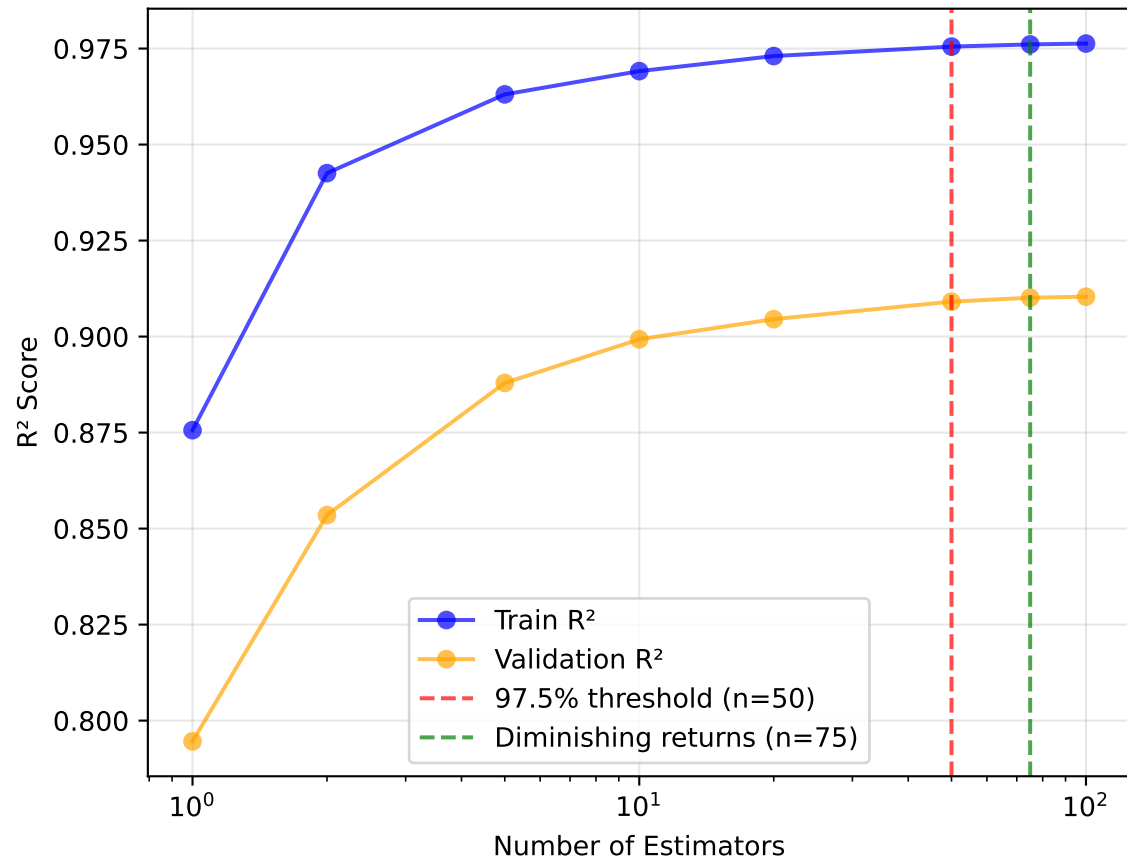
R 2 vs Number of Estimators
