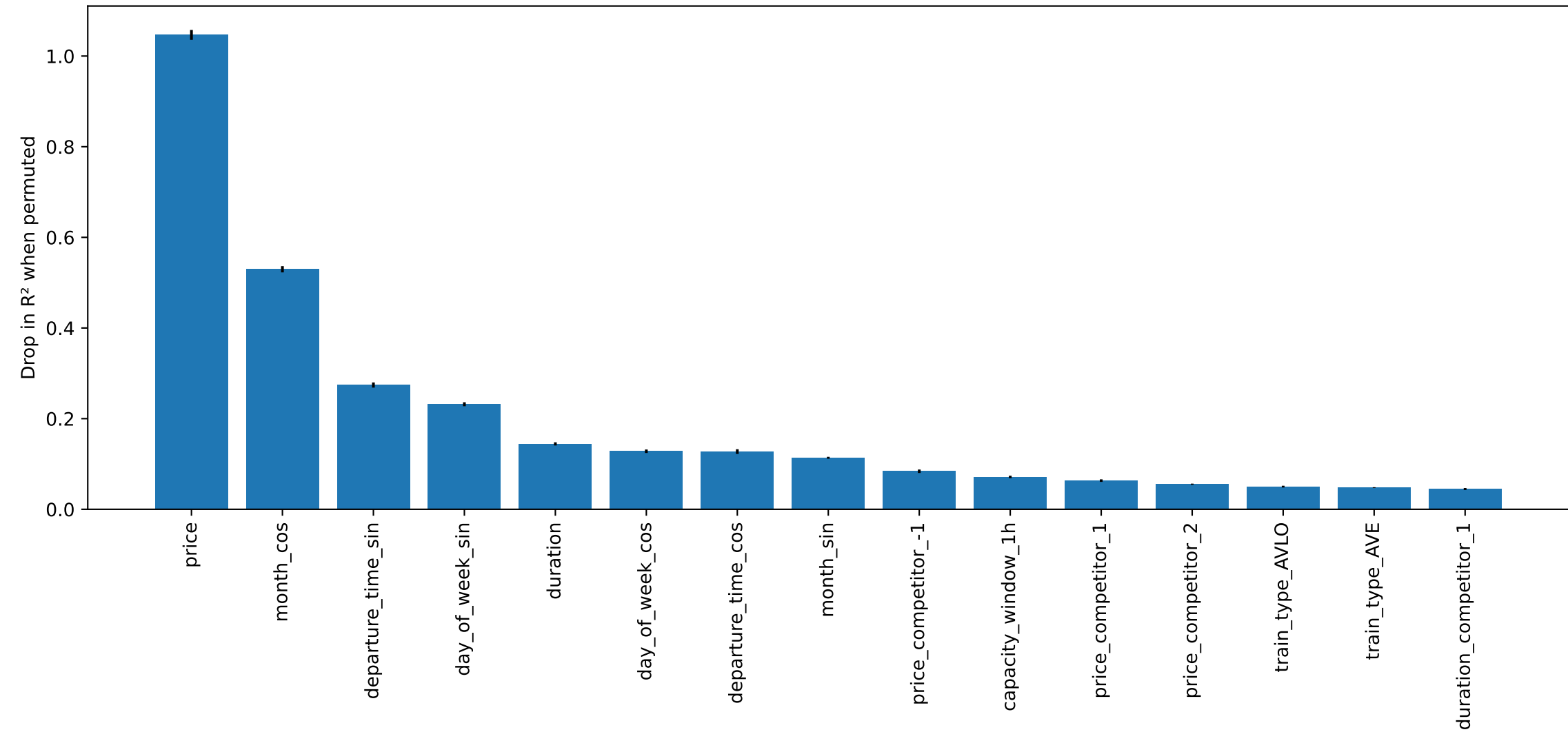
Decision Tree: Top 15 Permutation Feature Importances
