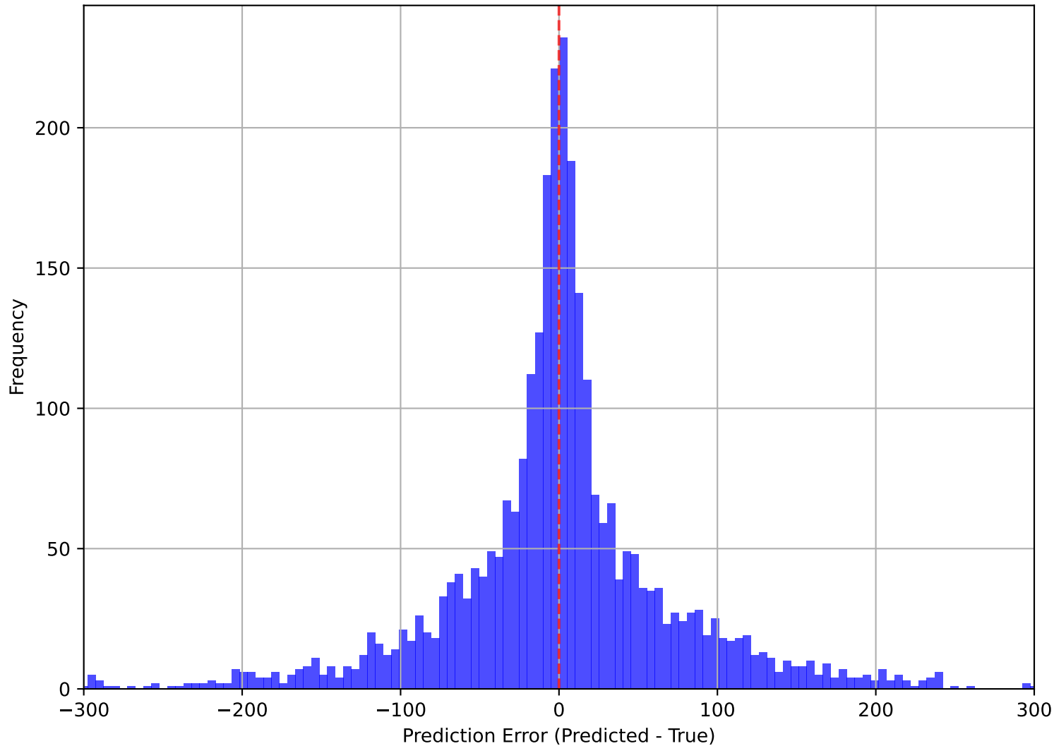
GBM: Histogram of Prediction Errors
