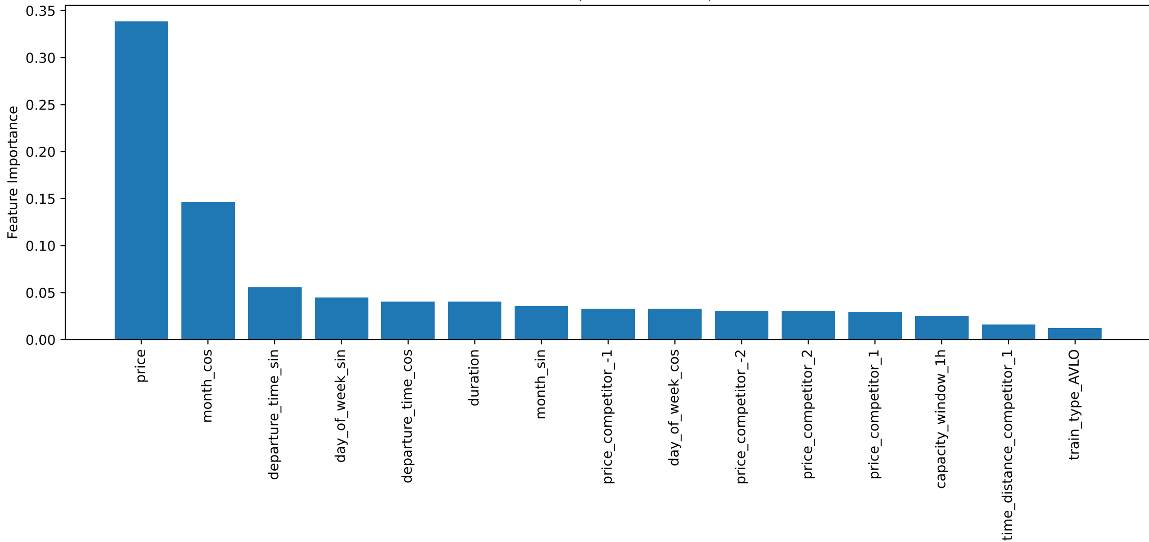
Random Forest: Top 15 Feature Importances
