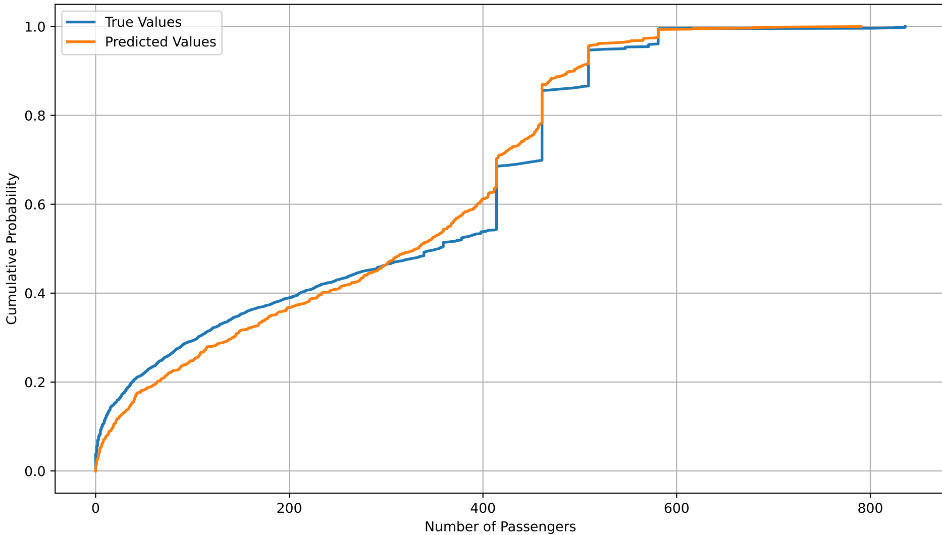
Decision Tree: Empirical CDF of True vs Predicted Values
