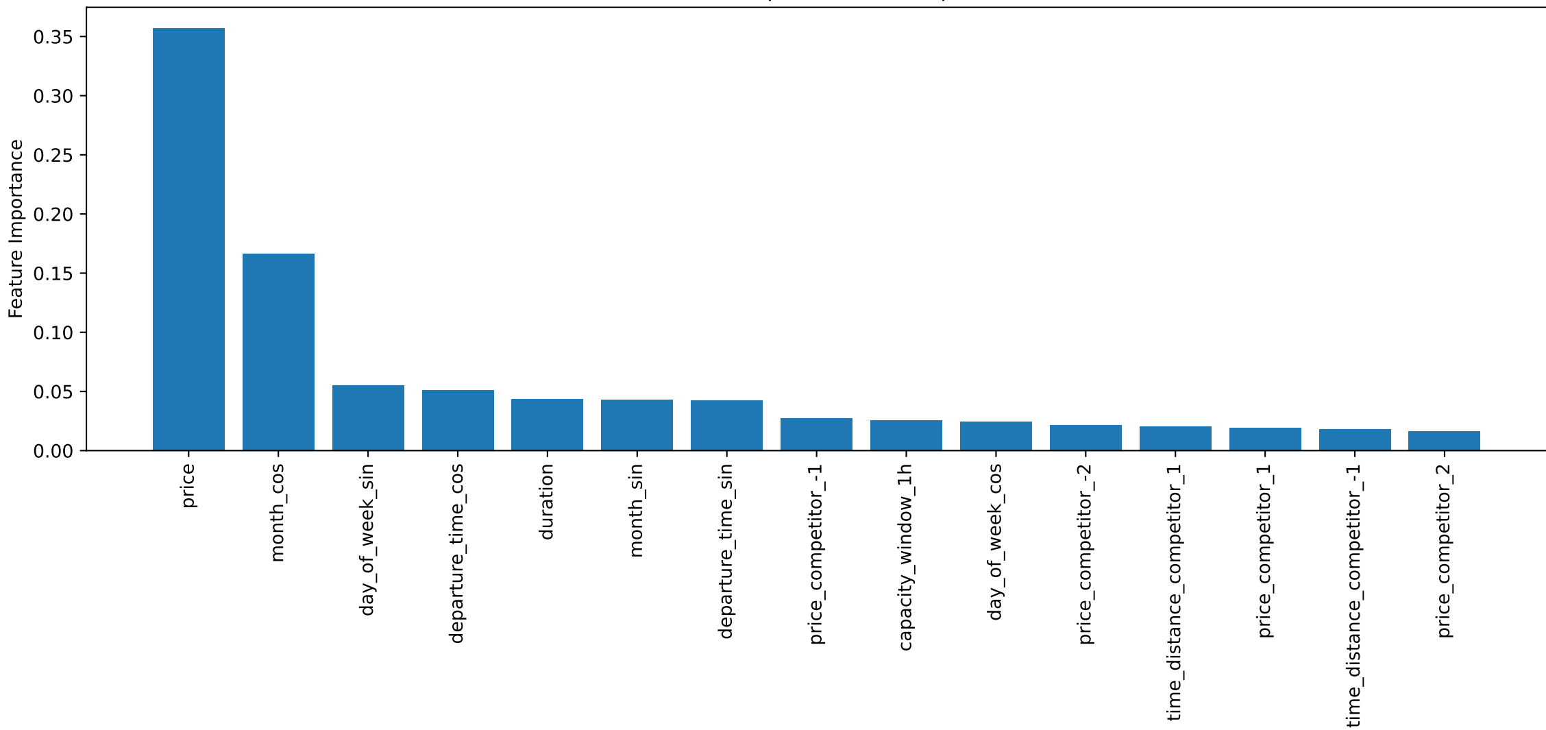
Decision Tree: Top 15 Feature Importances
