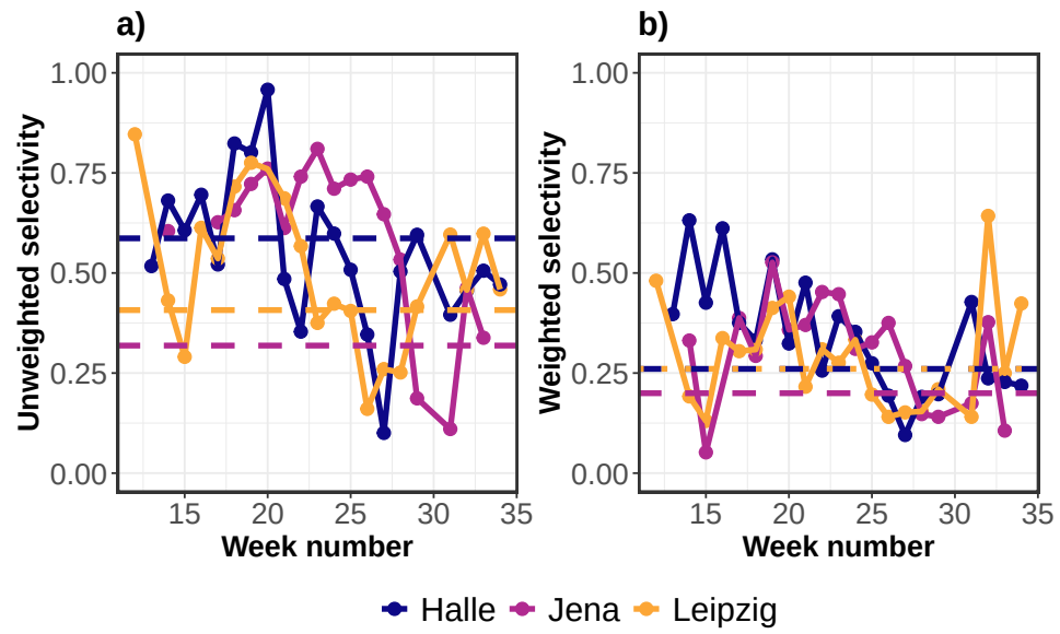
Figure S6. Temporal variation in mean pollinator selectivity across botanical gardens. Weekly mean selectivity (d') was calculated from interaction frequency matrices (a) and after accounting for floral resource availability (b).
