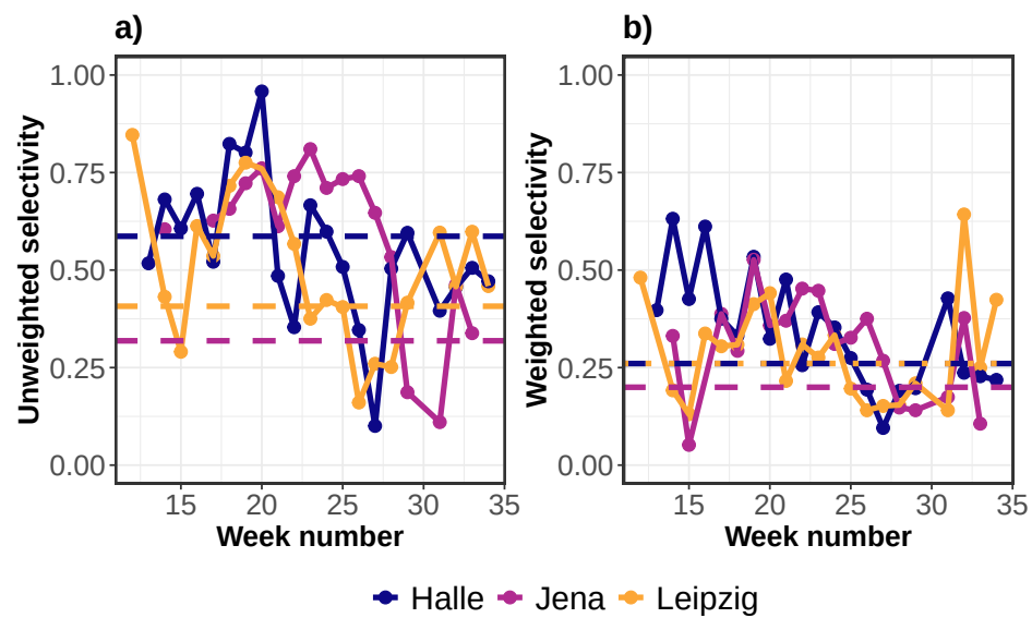
Figure S7. Temporal variation in mean pollinator selectivity across botanical gardens. Weekly mean selectivity ( d' ) was calculated from interaction frequency matrices (a) and after accounting for floral resource availability (b).
