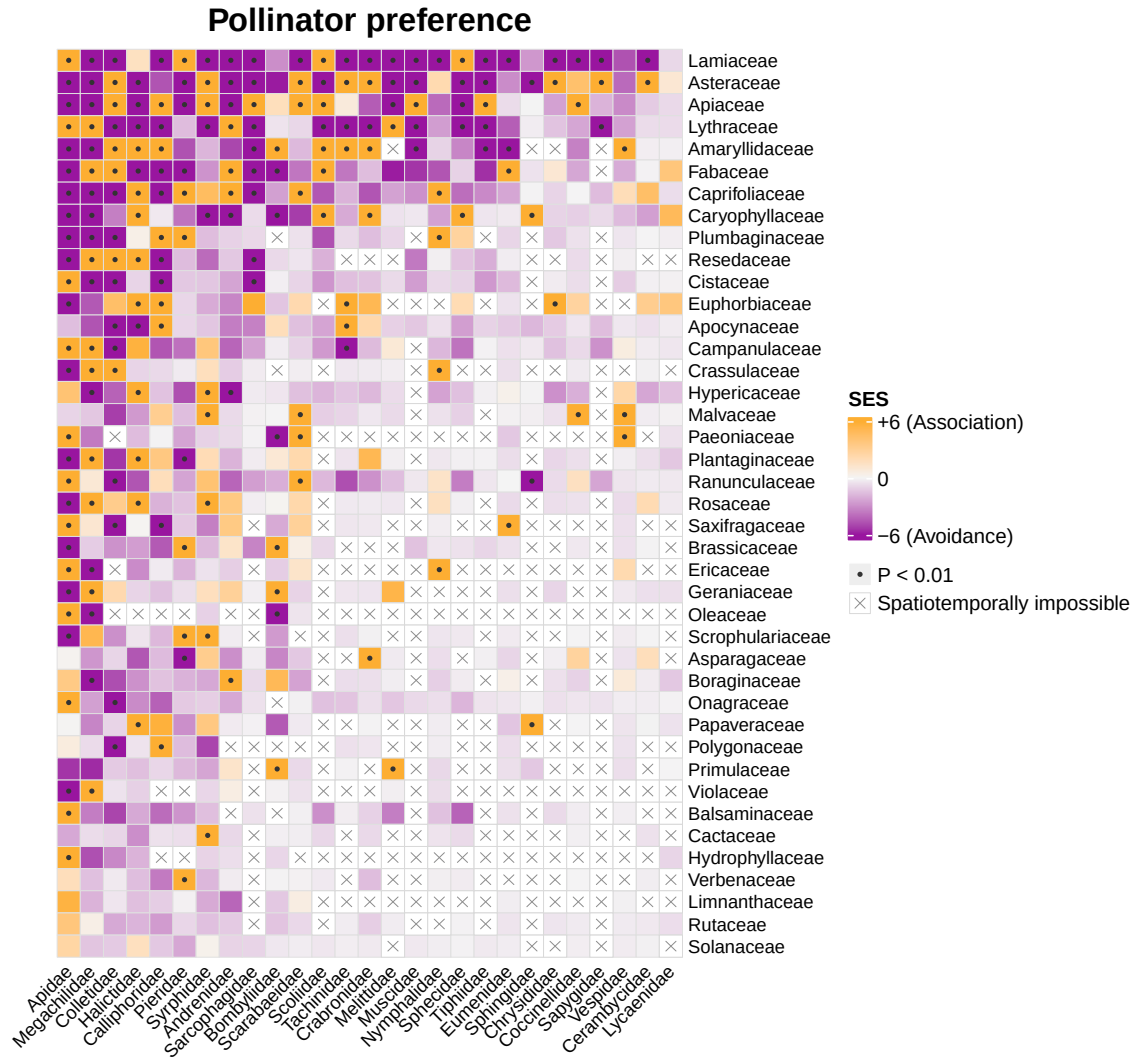
Figure 5. Heatmap of standardized effect sizes (SES) comparing observed plant-pollinator interactions at the family level with expectations from a spatiotemporally constrained null model. Purple indicates avoidance and orange indicates association relative to the null expectation. Black dots denote significant deviations from the null model ( p < 0.01 ). Crossed white cells indicate plant-pollinator family pairs that never co-occurred within the same garden and sampling week.
