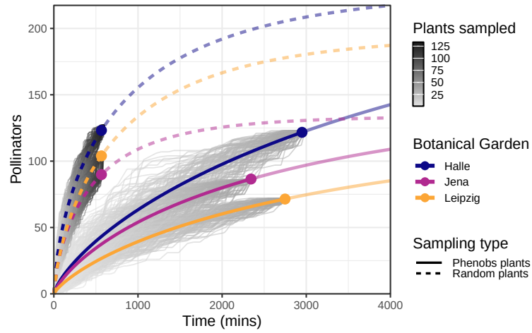
Figure 1: Figure S3. Accumulation curves of pollinator species across botanical gardens and sampling methods (dashed and solid lines). Each grey line represents one iteration of the accumulation curve, with a total of 100 iterations per garden and sampling method. The coloured lines represent the rarefied mean accumulation curves, with the dot indicating the total number of observed species. The segments of the lines extending beyond the dot represent the extrapolated number of expected species.
