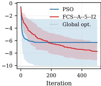
F21 (Shekel m = 5 )
