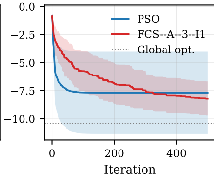
F22 (Shekel m = 7 )
