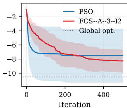
F23 (Shekel m = 10 )
