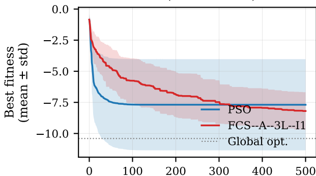
F22 (Shekel m = 7 )
