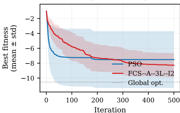
F23 (Shekel m = 10 )
