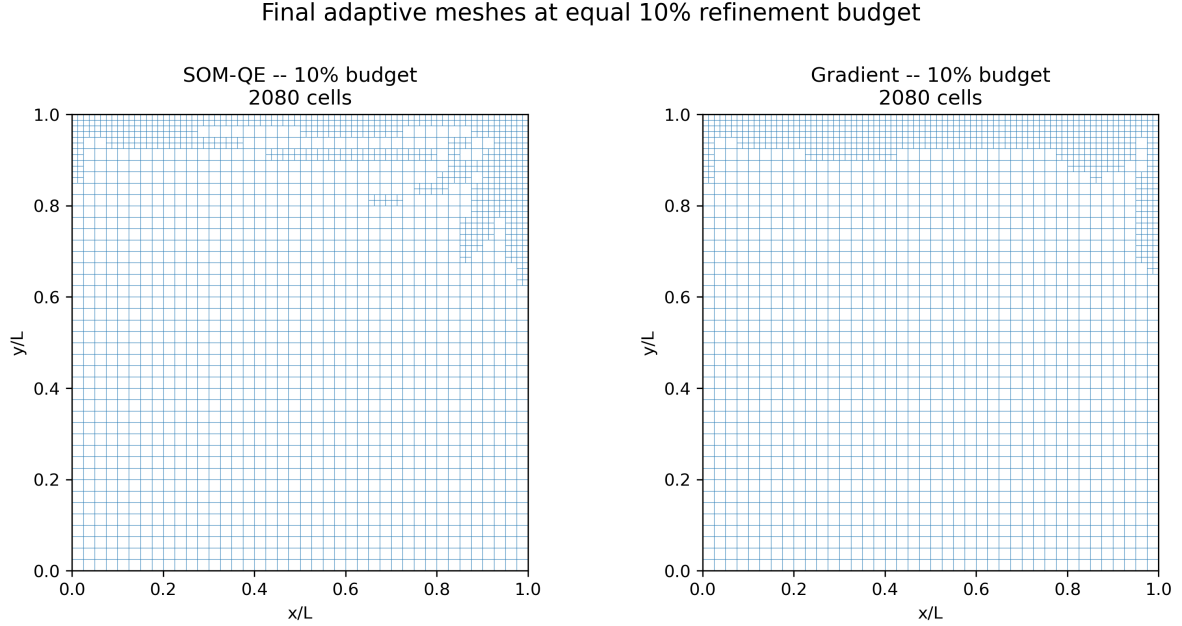
Figure 7: Final adaptive meshes obtained with SOM-QE and Gradient refinement at the same 10% refinement budget. Both meshes contain 2080 cells. The comparison therefore isolates differences in the spatial allocation of refinement rather than differences in total cell count.
