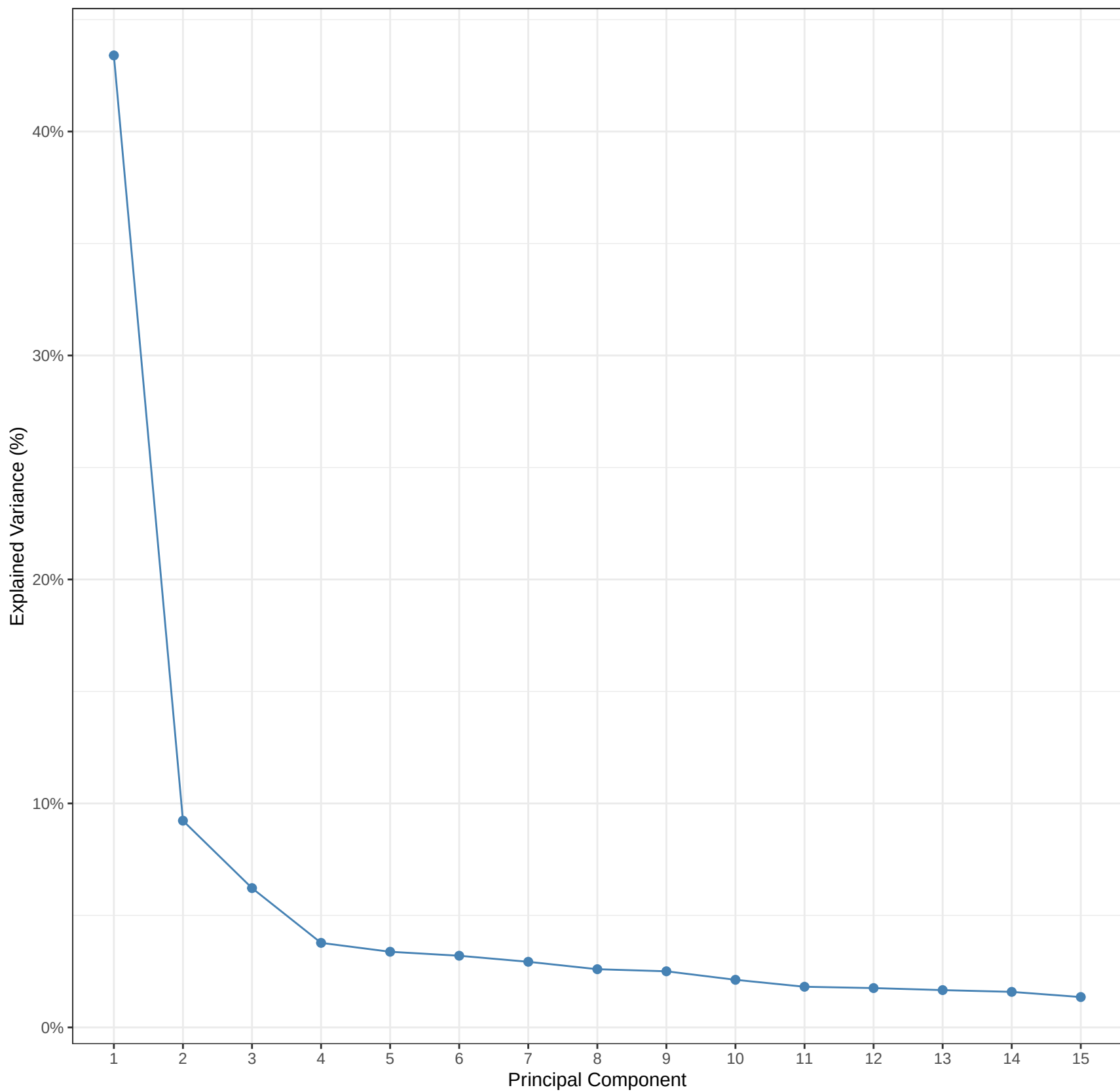
Scree Plot
