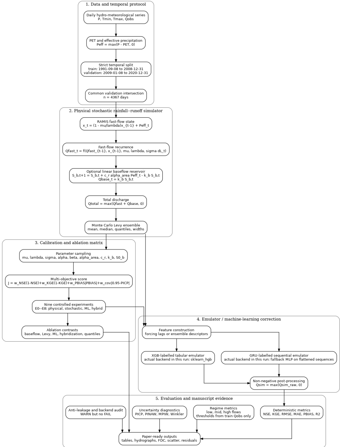
Figure 1: StoHyMoLAP workflow from daily hydro-meteorological data to lumped physical simulation, Lévy-type stochastic ensemble generation, ensemble-descriptor construction, ML emulation, ablation comparison and audit-controlled manuscript evidence.
