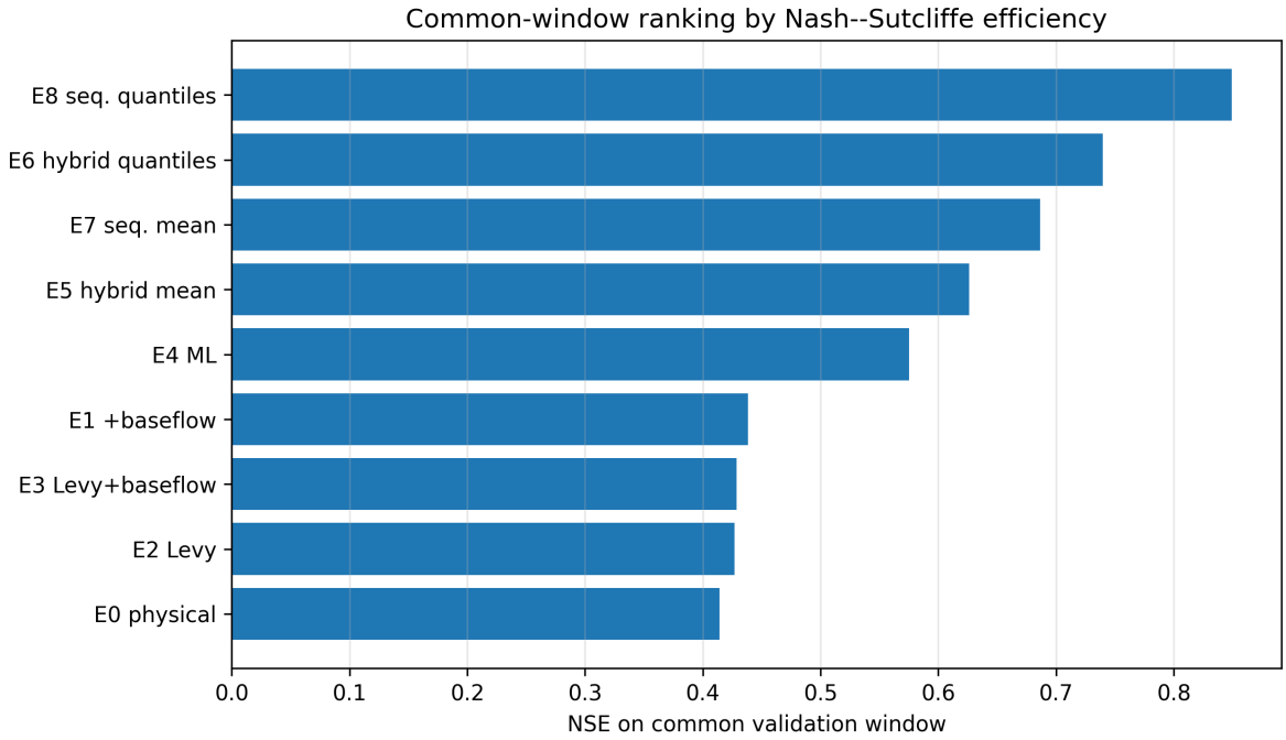
Figure 2: Ranking of experiments by common-window NSE. Numerical values correspond to Table 2; the GRU-labelled entries should be interpreted with the backend audit because they executed as fallback MLP models.
