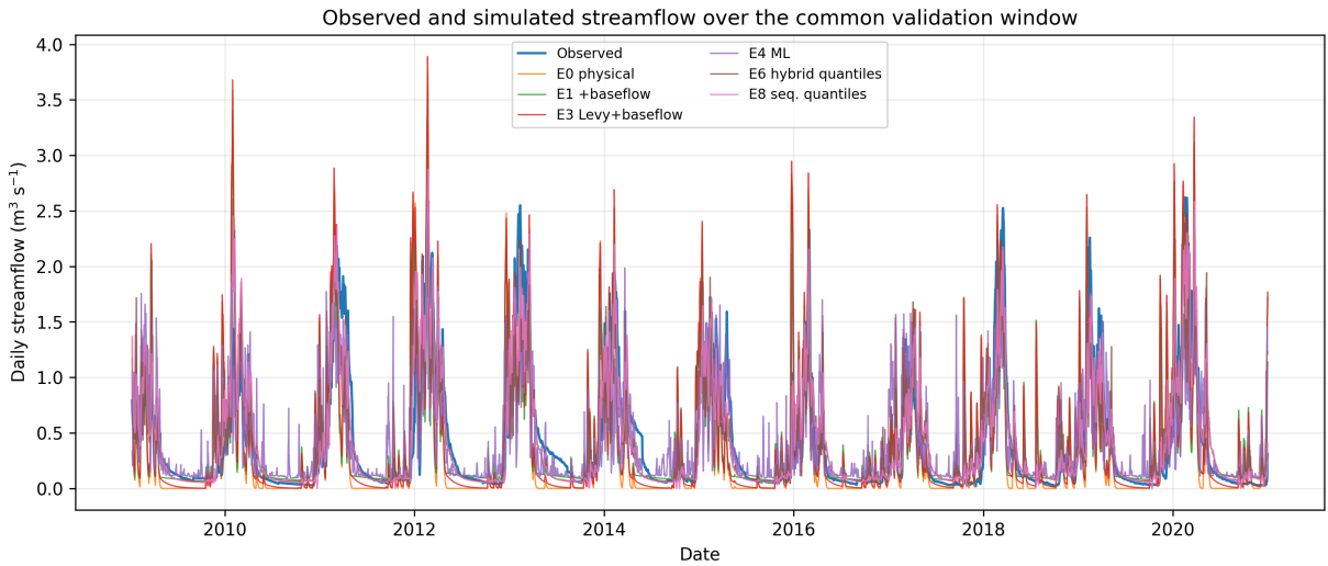
Figure 3: Observed and simulated daily discharge ( \text{m}^3 \text{s}^{-1} ) over the common validation window for representative physical, pure ML and hybrid models.
