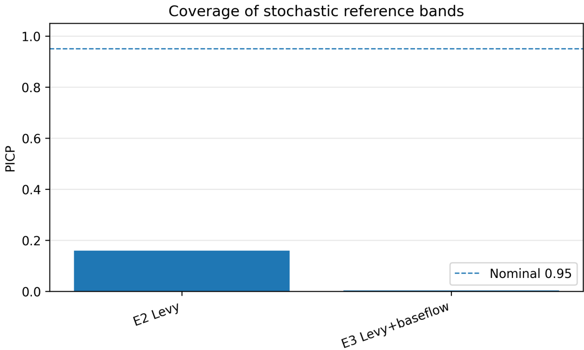
Figure 7: Prediction interval coverage probability for nominal 95% stochastic physical reference intervals. The dashed line marks the nominal 0.95 coverage target.
