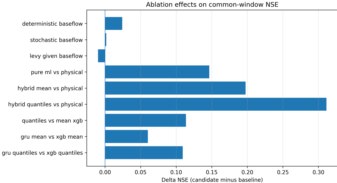
Figure 5: Ablation effects expressed as candidate-minus-baseline \Delta\text{NSE} . Numerical values are reported in Table 3; GRU-labelled contrasts refer to fallback-MLP execution in the current evidence package.
