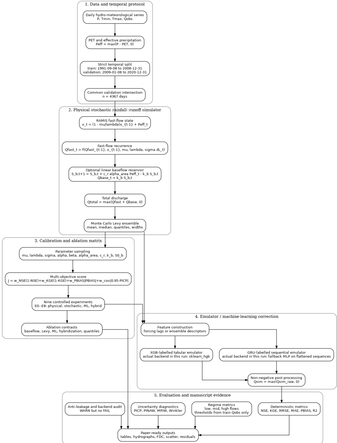
Figure 1: StoHyMoLAP workflow used in this study. Daily hydro-meteorological inputs are converted into lumped RAMIS simulations, Lévy-type stochastic physical ensembles, ensemble descriptors and ML estimates; the final step applies common-window evaluation and audit checks.
