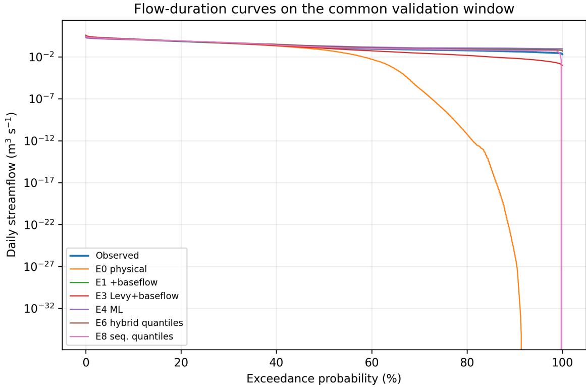
Figure 4: Flow-duration curves for observed and simulated daily discharge ( \text{m}^3 \text{s}^{-1} ) over the common validation window.
