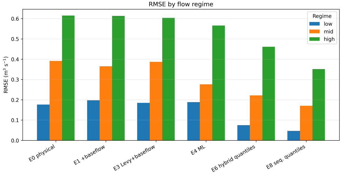
Figure 6: RMSE ( \text{m}^3 \text{s}^{-1} ) by low-, mid- and high-flow regimes for representative models. Values correspond to Table 4.
