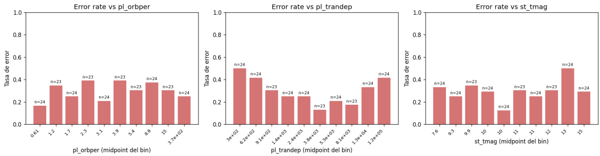
Figure 3: Error rate vs. binned period, transit depth and stellar magnitude. Errors concentrate in shallow transits near the noise floor.
