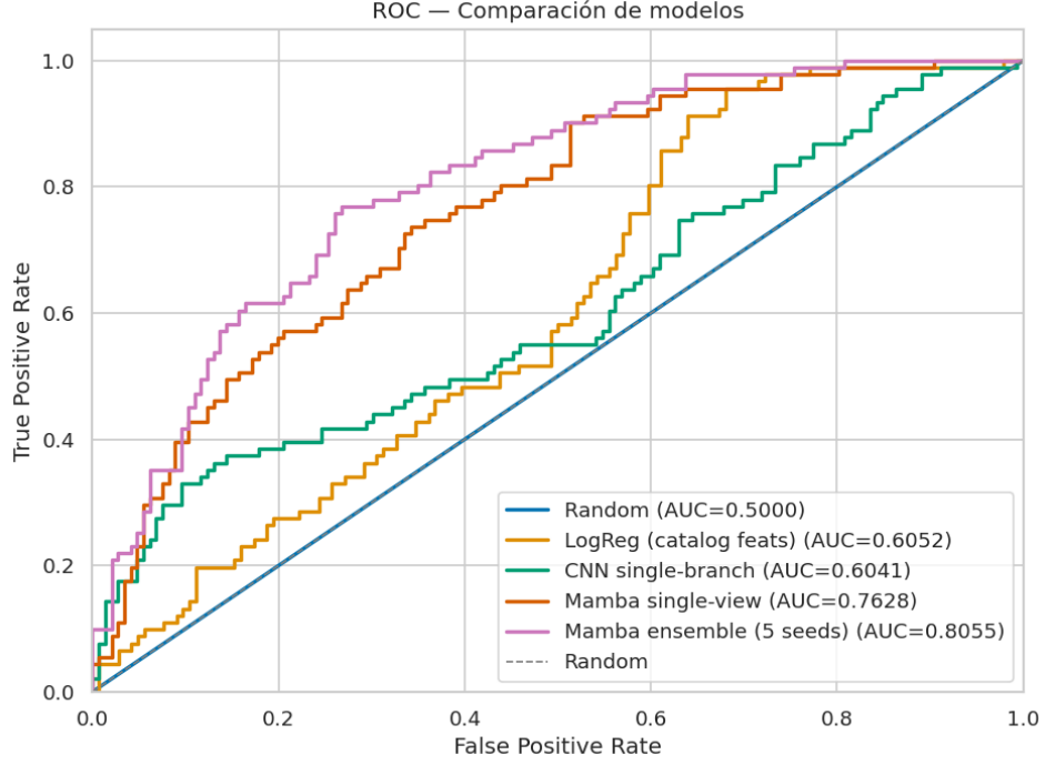
Figure 1: Test ROC curves for the global-view models. Mamba (upper-left) is clearly separated from the CNN and logistic regression (near the diagonal); the visual gap is the +0.20 AUC difference quantified in Table 3.
