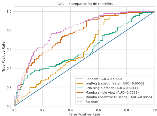
Fig. 1. Test ROC curves for the global-view models. Mamba (upper-left) is clearly separated from the CNN and logistic regression (near the diagonal); the visual gap is the +0.20 AUC difference quantified in Table III.
