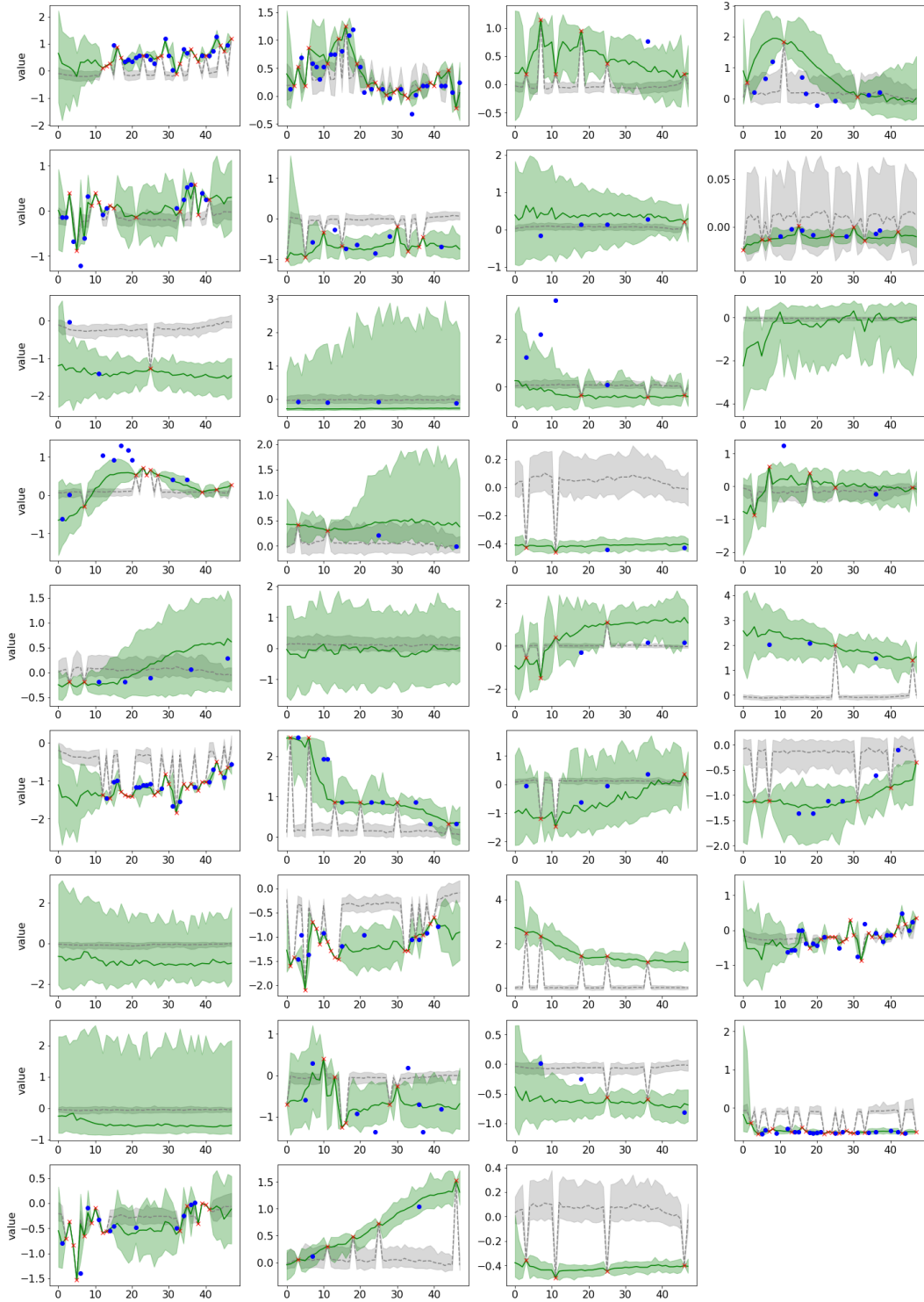
Figure 9: Comparison of imputation between GP-VAE and CSDI for the healthcare dataset (50% missing). The result is for time series sample with all 35 features. The red crosses show observed values and the blue circles show ground-truth imputation targets. Green and gray colors correspond to CSDI and GP-VAE, respectively. For each method, median values of imputations are shown as the line and 5% and 95% quantiles are shown as the shade.
