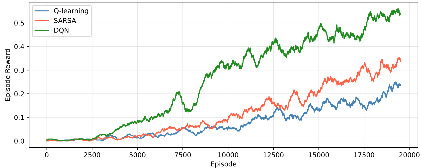
Episode Reward — 8×8 Slippy: Q-learning vs SARSA vs DQN
