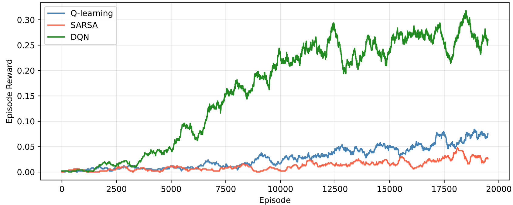
Episode Reward — 8×8 Slippery: Q-learning vs SARSA vs DQN
