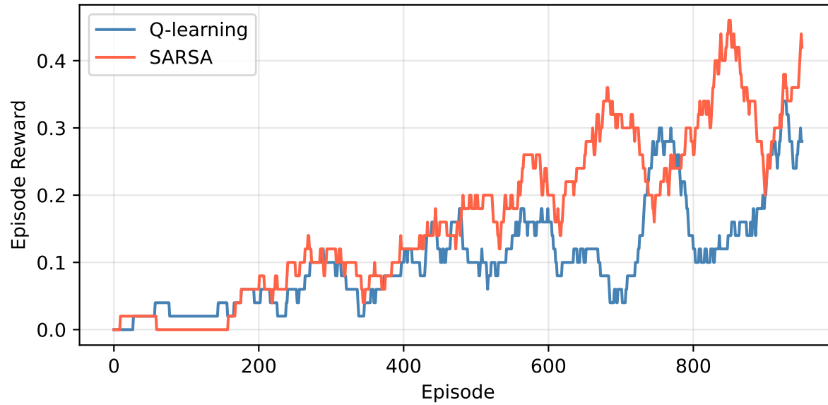
4x4 (non-slippery)
