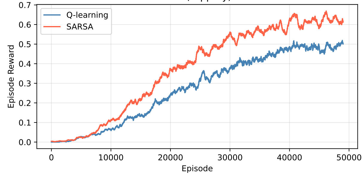
8x8 (slippery)
