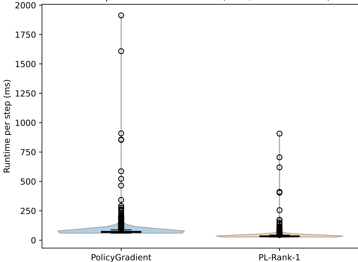
Per-Step Runtime Distribution (DCG, MSLR-WEB10k)
