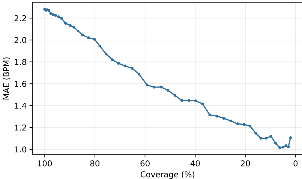
HeartV6 confidence--coverage trade-off
