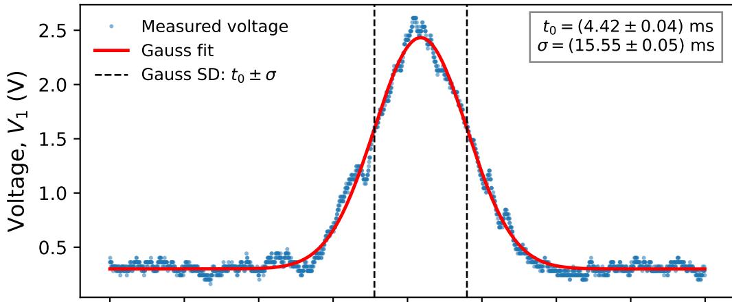
Proton Spin-Echo Envelope (Channel 1)
