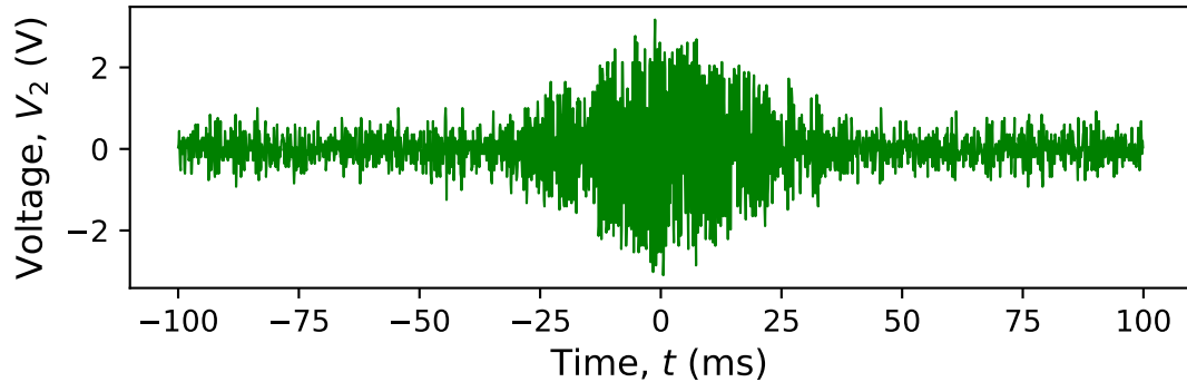
Proton-Precession Signal (Channel 2)
