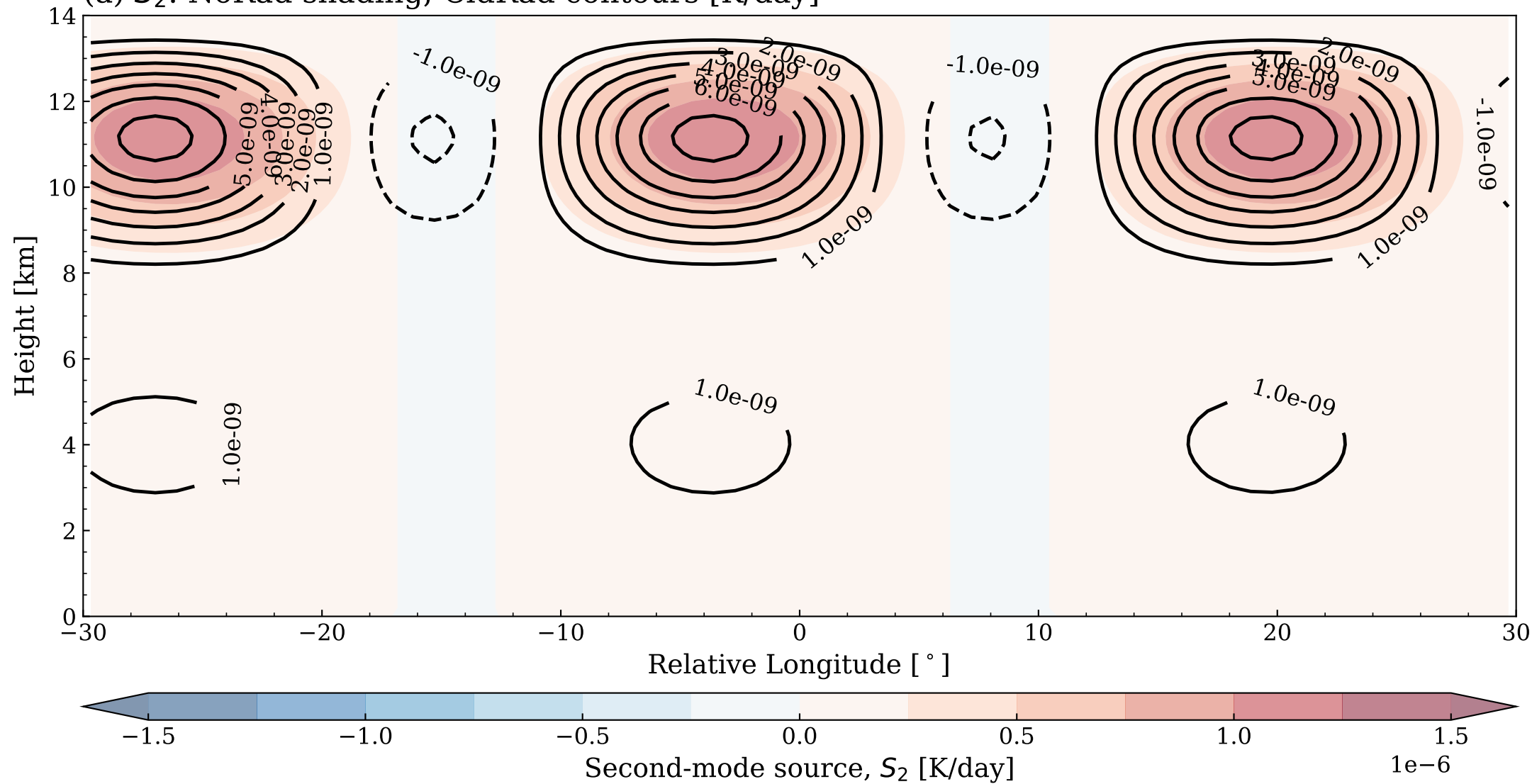
(a) S_2 : NoRad shading; CldRad contours [K/day]
