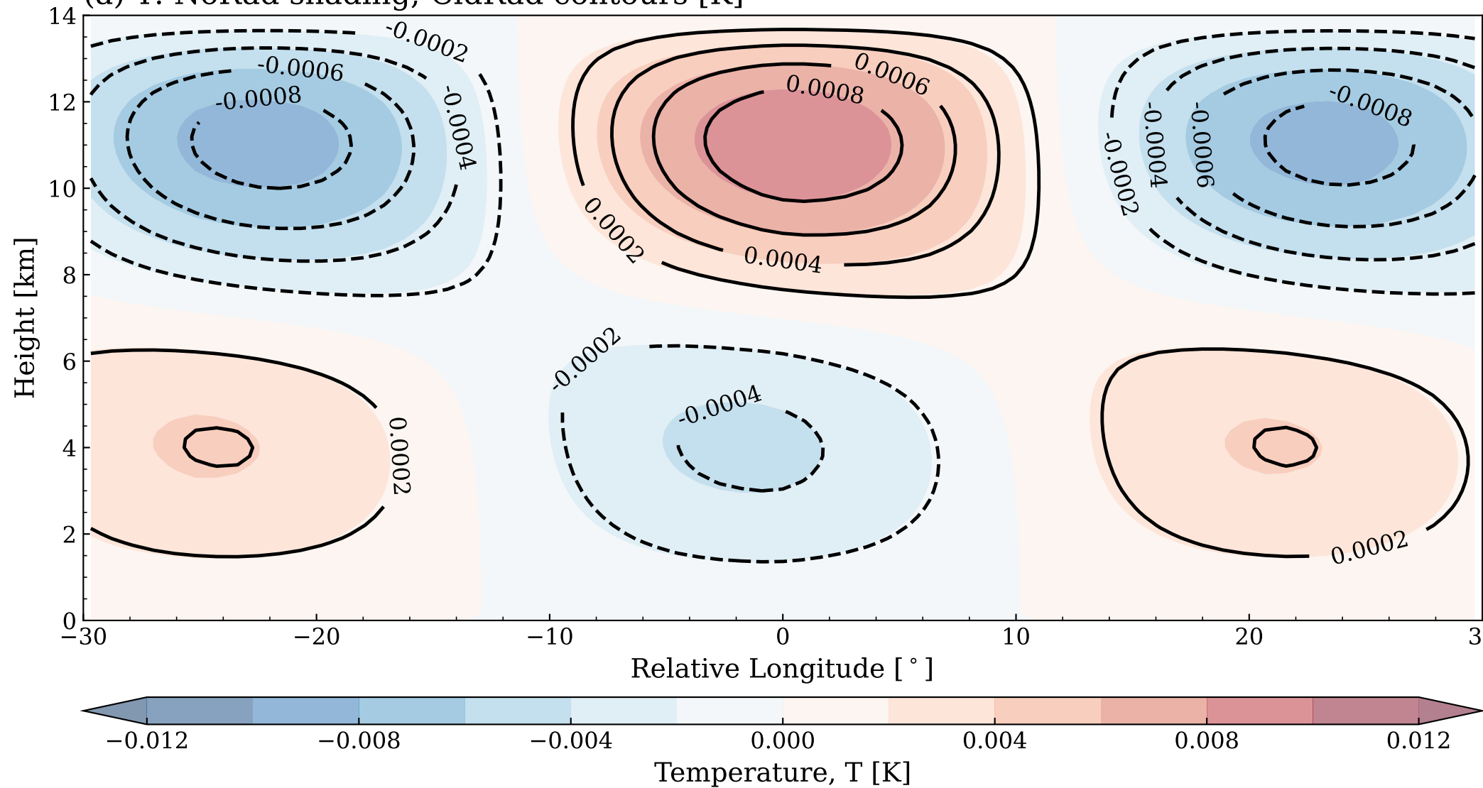
(a) T: NoRad shading; CldRad contours [K]
